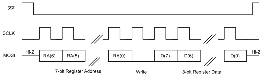
Figure 26. SPI Write
