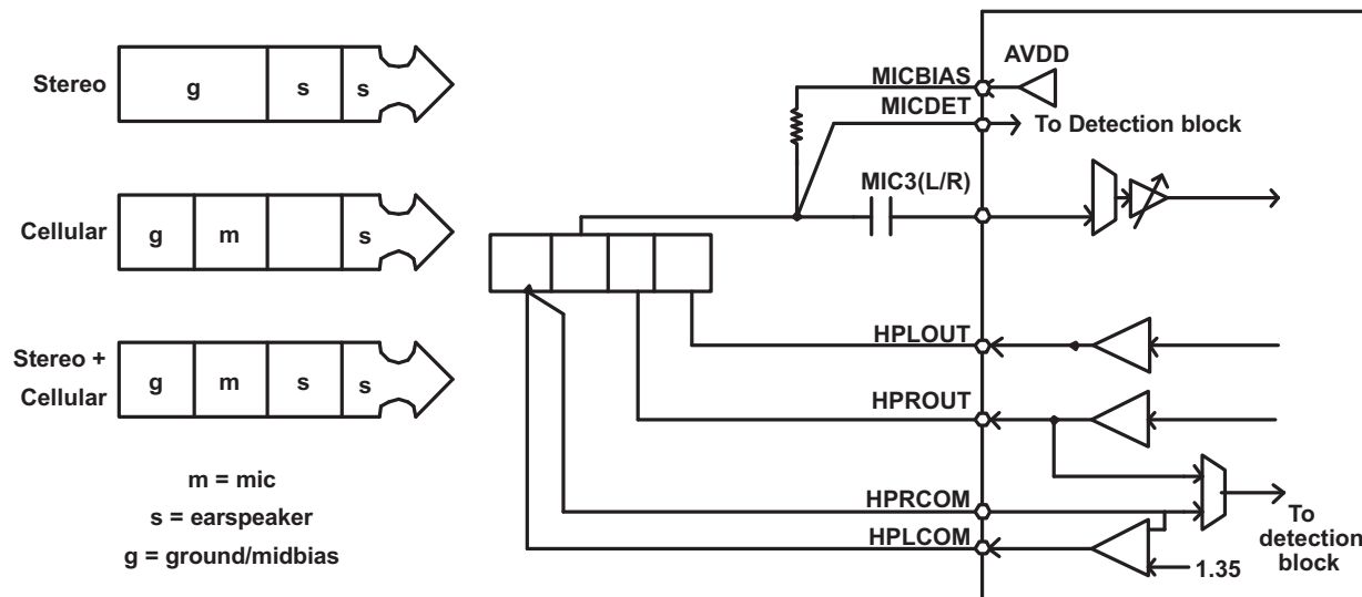
Figure 21. Configuration Of Device For Jack Detection Using A Pseudo-Differential (Capless) Headphone Output Connection
