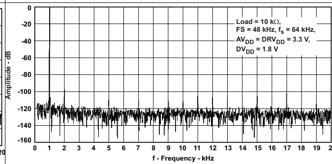
Figure 10. Right DAC FFT
