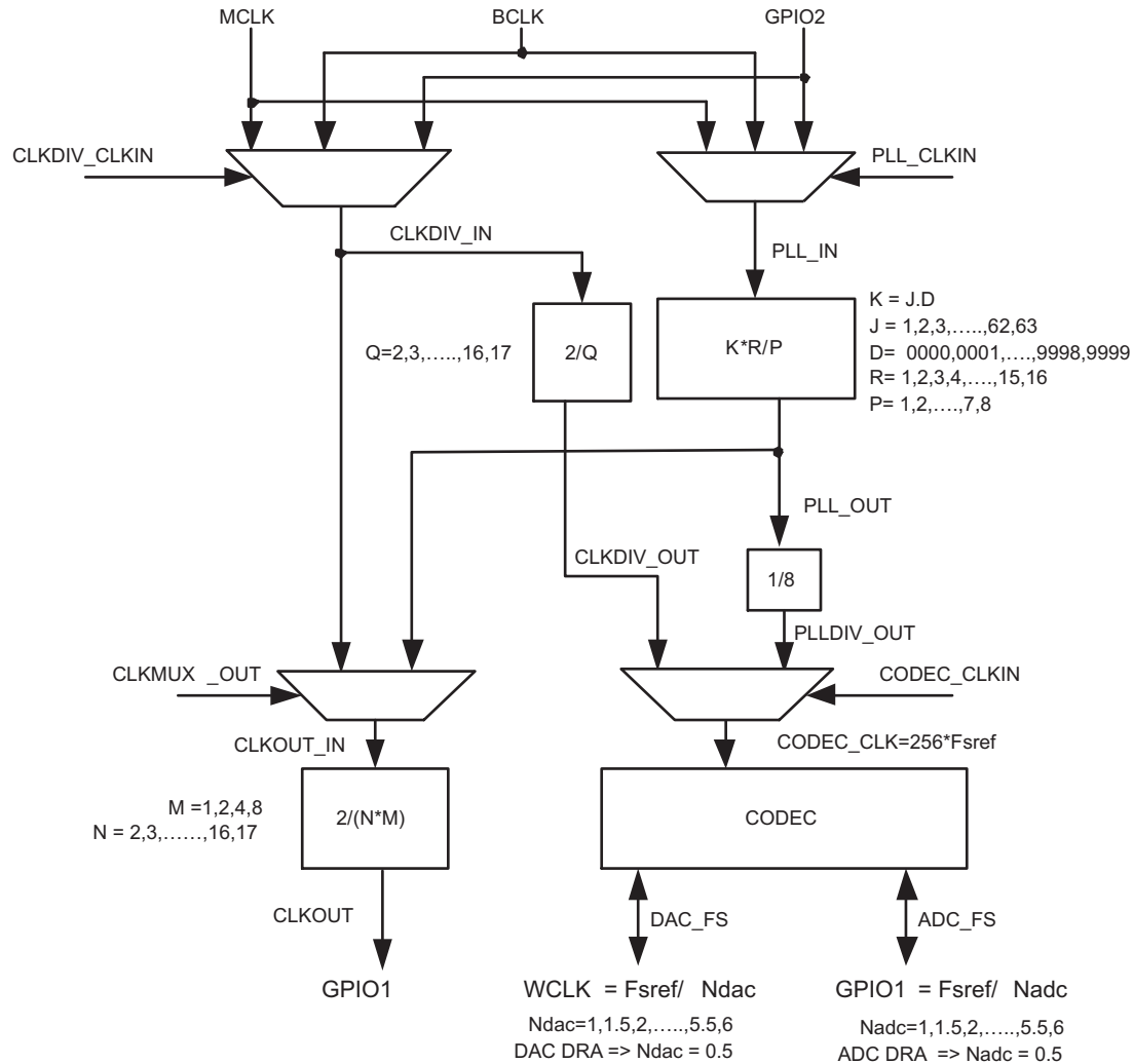
Figure 38. Audio Clock Generation Processing
