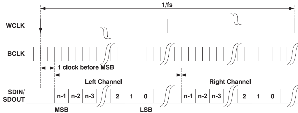
Figure 35. I²S Serial Data Bus Mode Operation
