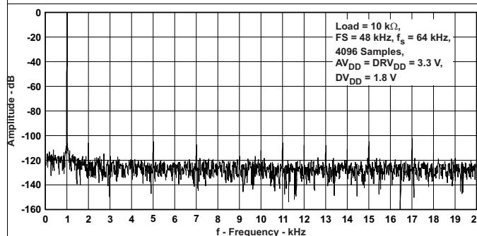
Figure 9. Left DAC FFT
