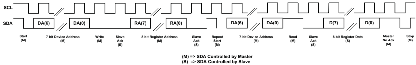
Figure 30. I²C Read
