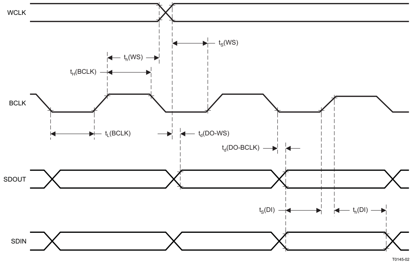
Figure 2. I²S/LJF/RJF Timing In Slave Mode
