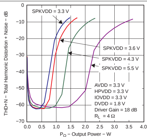
Figure 5-16. Total Harmonic Distortion + Noise vs Output Power Class-D Speaker-Driver Output Power (RL = 4 Ω)
