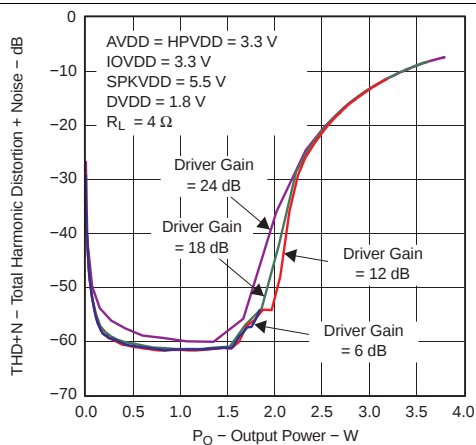
Figure 5-15. Total Harmonic Distortion + Noise vs Output Power Max Class-D Speaker-Driver Output Power (RL = 4 Ω)
