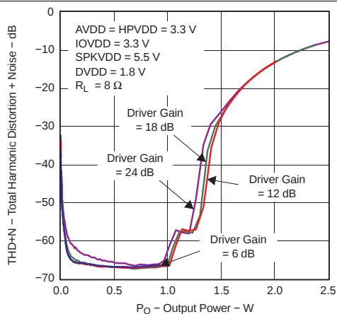
Figure 5-17. Total Harmonic Distortion + Noise vs Output Power Max Class-D Speaker-Driver Output Power (RL = 8 Ω)
