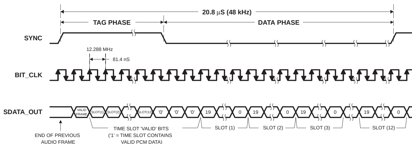
Figure 9. AC-Link Serial Interface Protocol Output Frame
