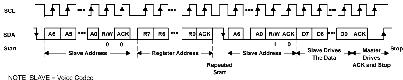
Figure 2. I²C Read From Voice Codec: Protocol A
