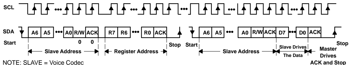
Figure 3. I²C Read From Voice Codec: Protocol B
