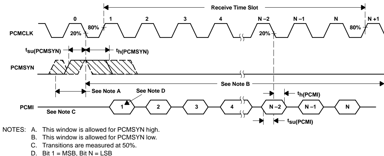
Figure 6. Receive Timing Diagram
