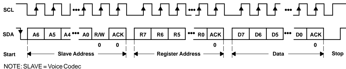
Figure 1. I²C-Bus Write to Voice Codec
