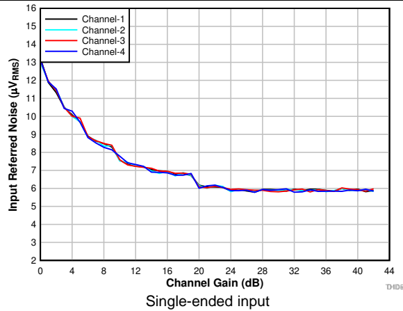
Figure 11. Input-Referred Noise vs Channel Gain
