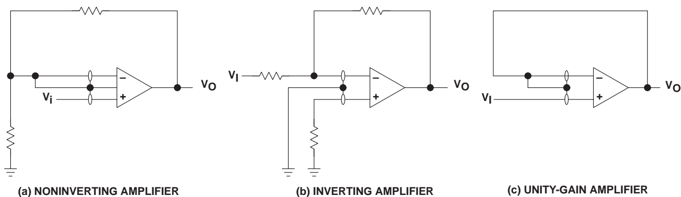
Figure 42. Guard-Ring Schemes
