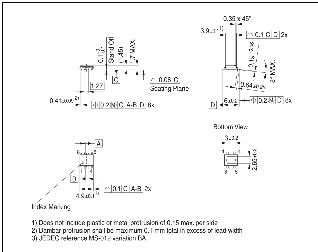
Figure 5 PG-DSO-8 EP
