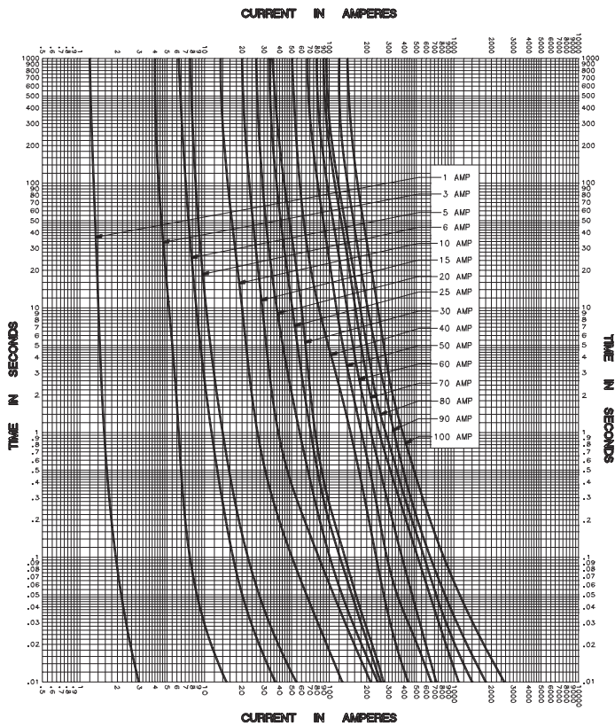
Time Curve for 1-100 Amps
