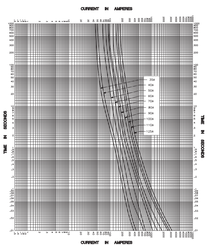
Time Curve for 35-125 Amps
