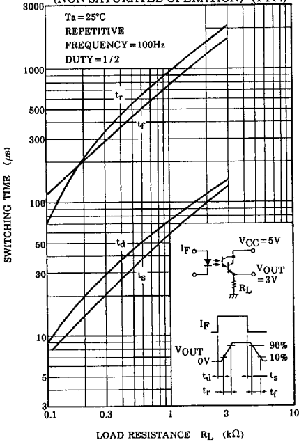
SWITCHING CHARACTERISTICS (NON SATURATED OPERATION) (TYP.)
