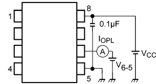
Fig. 13.1.2 I_{OPL} Test Circuit
