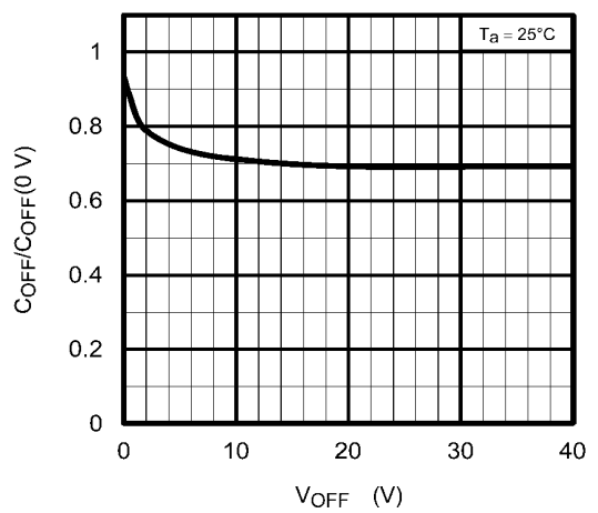
Fig. 12.1.11 C_{OFF}/C_{OFF}(0V) - V_{OFF}
