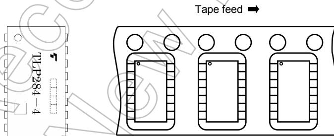
Figure 2 Device Orientation
