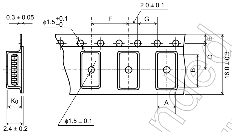
Figure 3 Tape Forms
