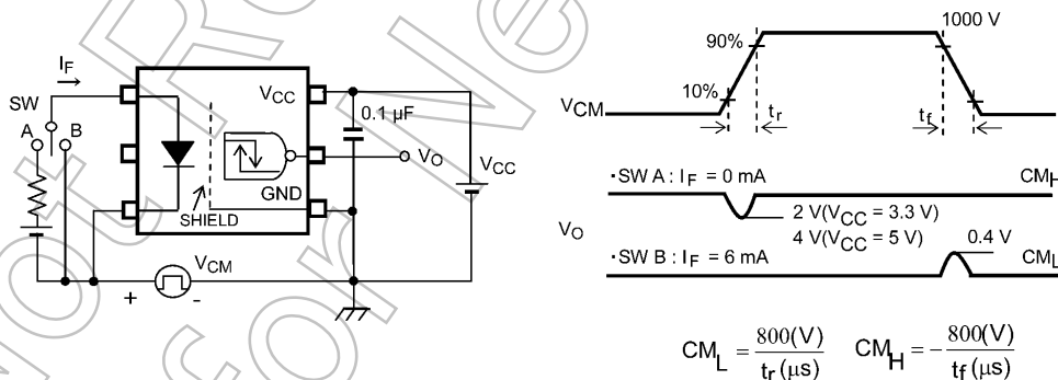
Fig. 12.1.6 Common-Mode Transient Immunity Test Circuit and Waveform
