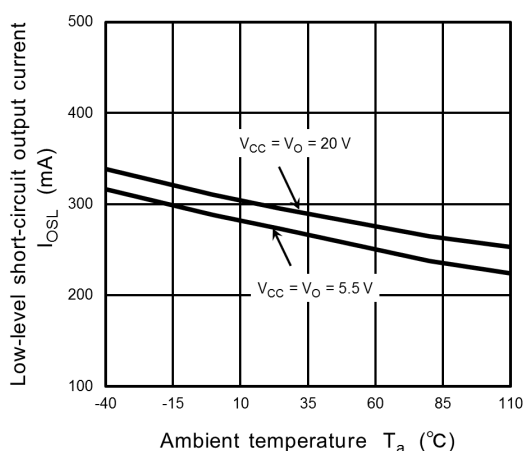
Fig. 13.2.9 I_{OL} - T_a
