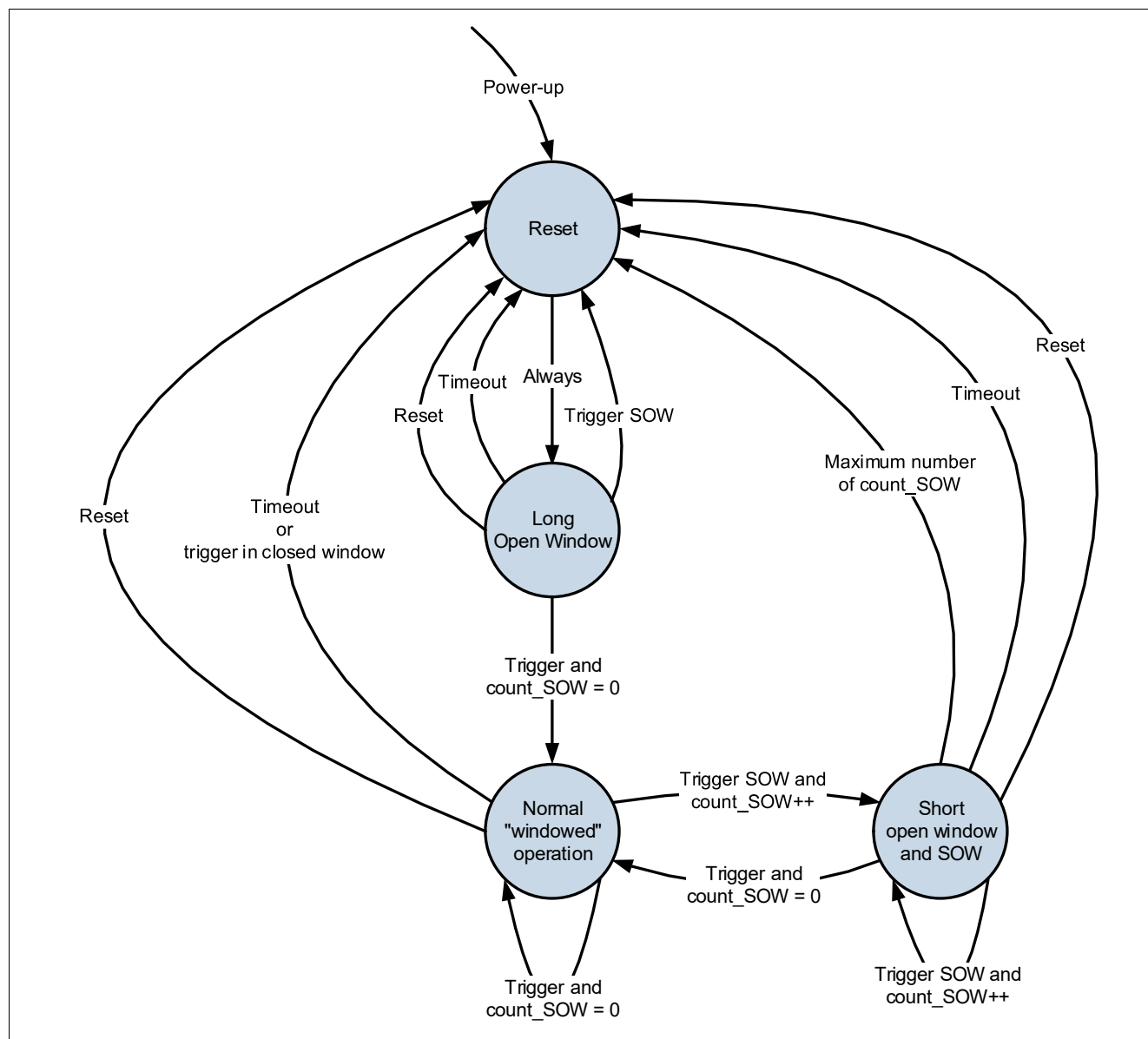
Figure 16 Watchdog timer behavior
