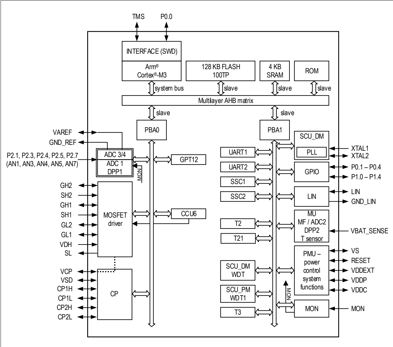
Figure 1 Block diagram
