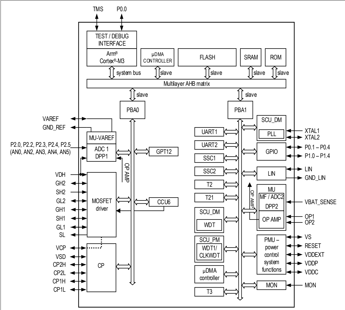
Figure 1 Block diagram
