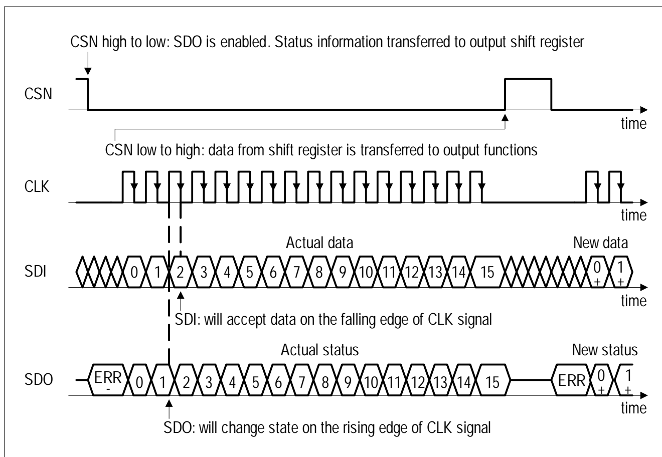
Figure 53 SPI Data Transfer Timing (note the reversed order of LSB and MSB shown in this figure compared to the register description)
