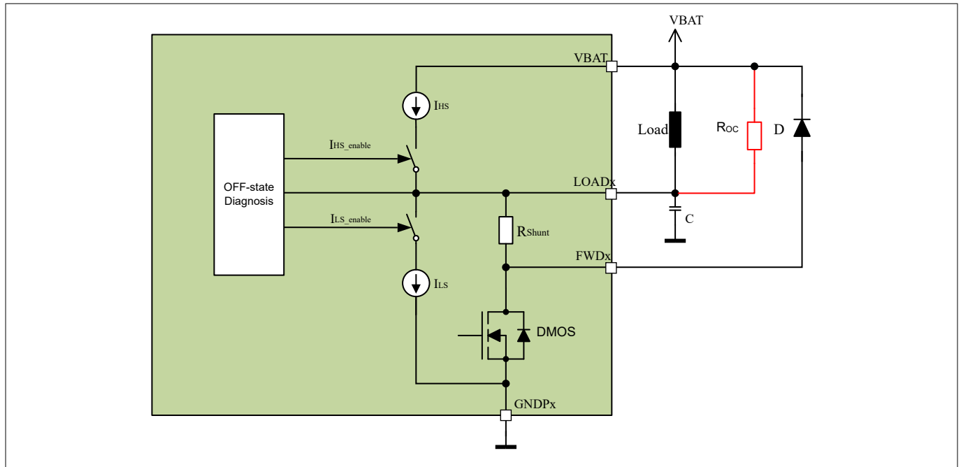
Figure 20 Overcurrent
