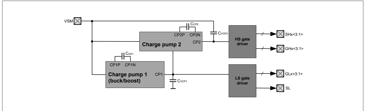
Figure 4 Power supply
