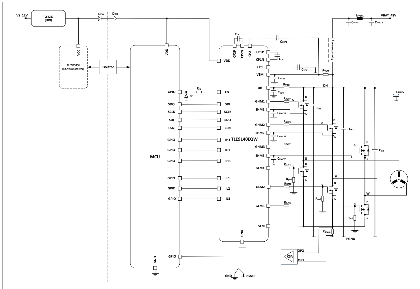
TLE9140EQW is driven by the general microcontroller for 48 V applications supply concept: isolated 12 V supply for the general MCU with diodes
