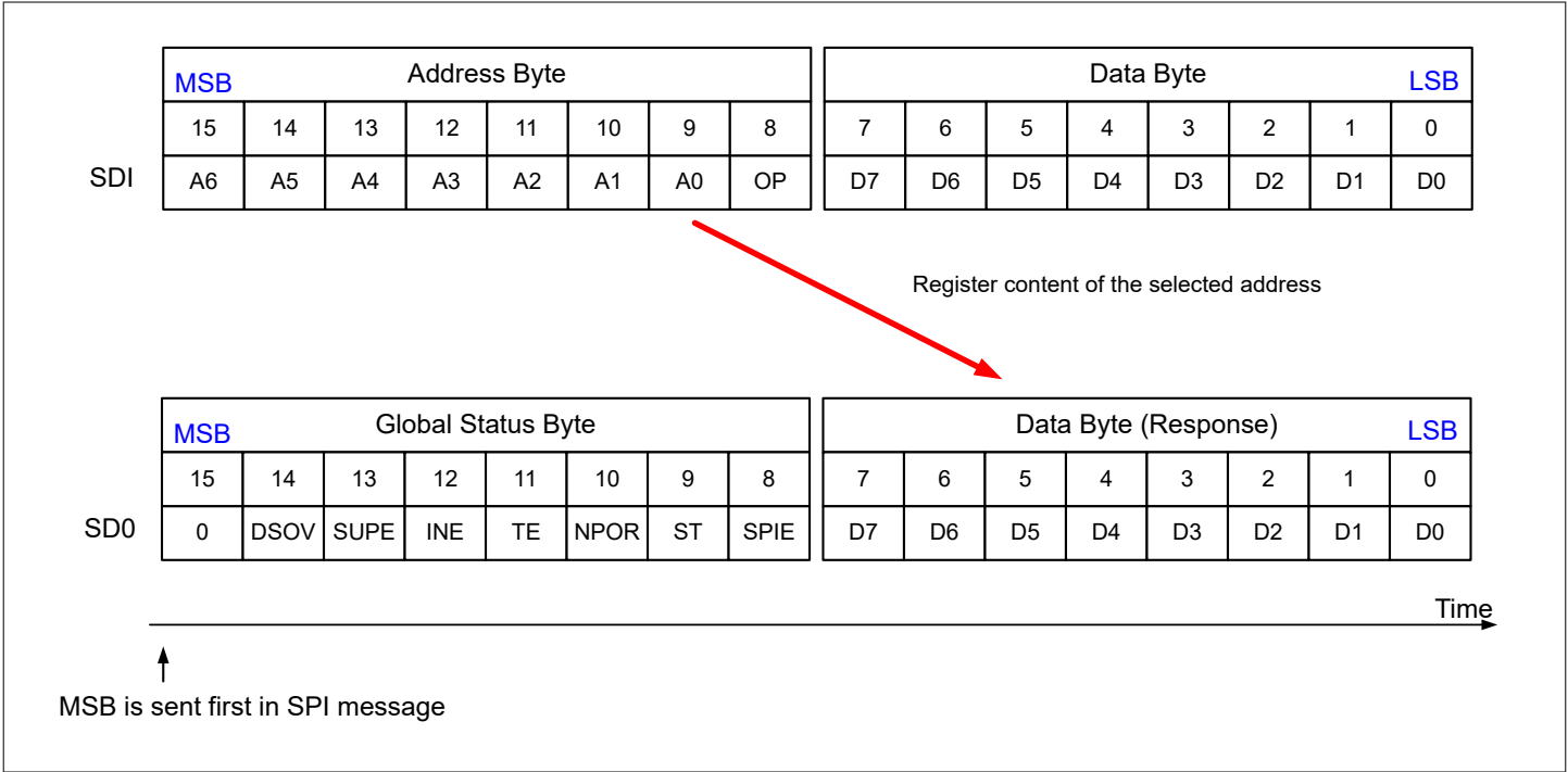
Figure 18 In-frame response
