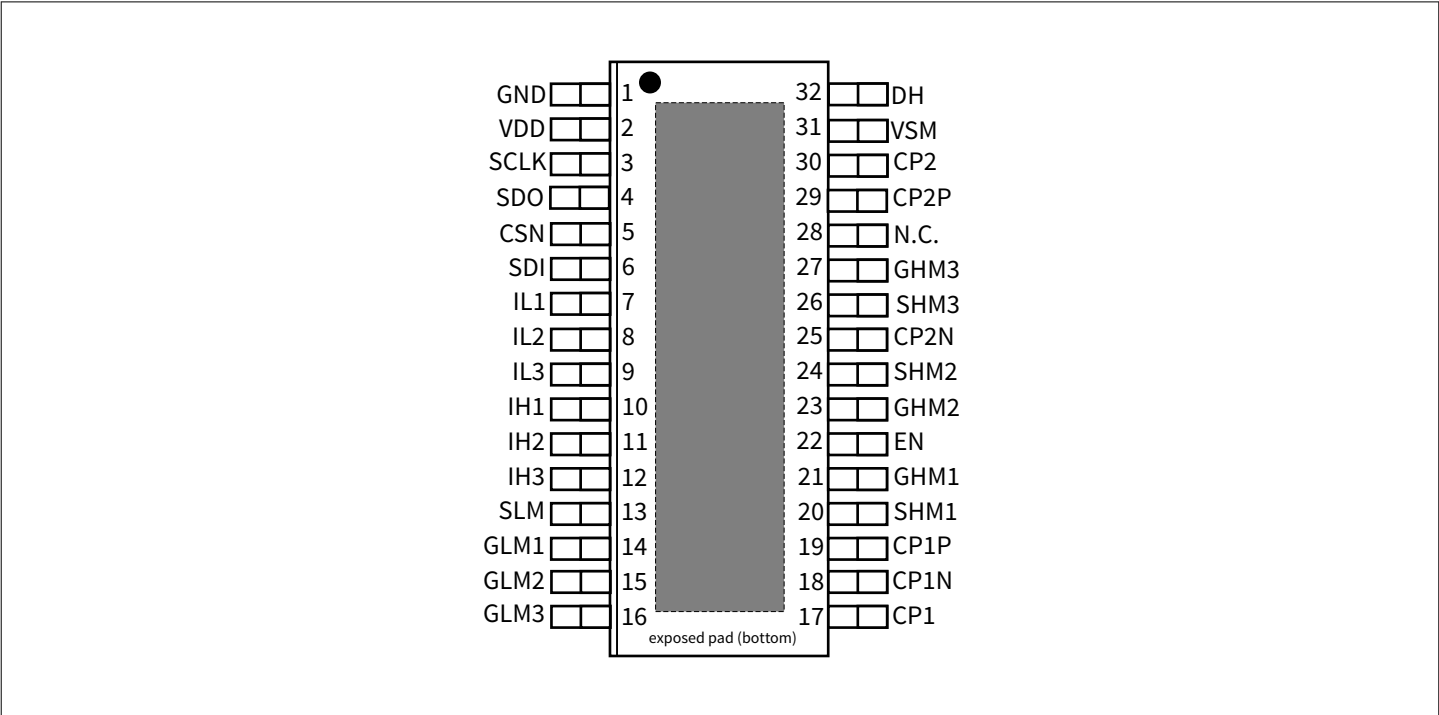
Figure 2 Pin configuration
