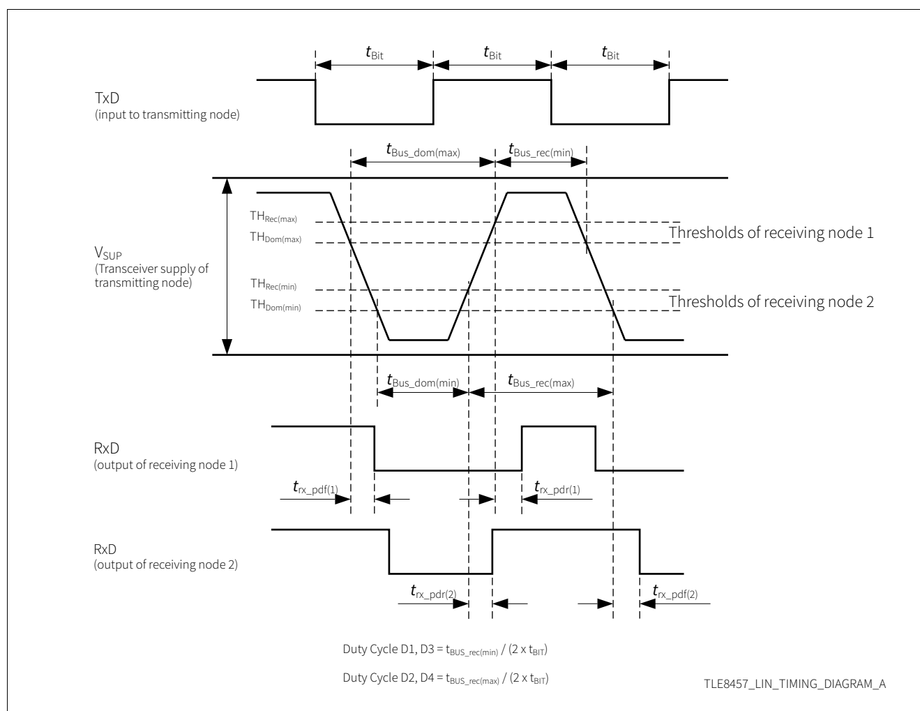
Figure 17 Timing diagram for dynamic transceiver characteristics
