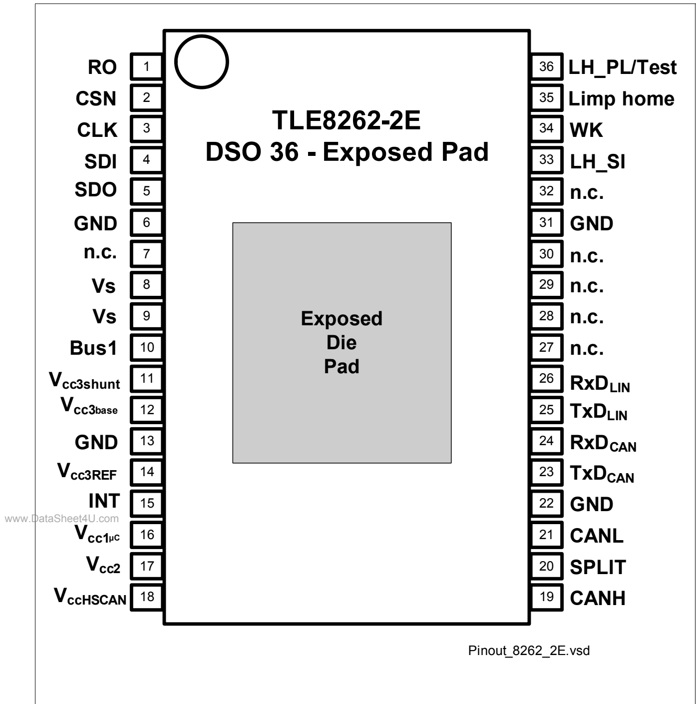
Figure 4 Pin Configuration
