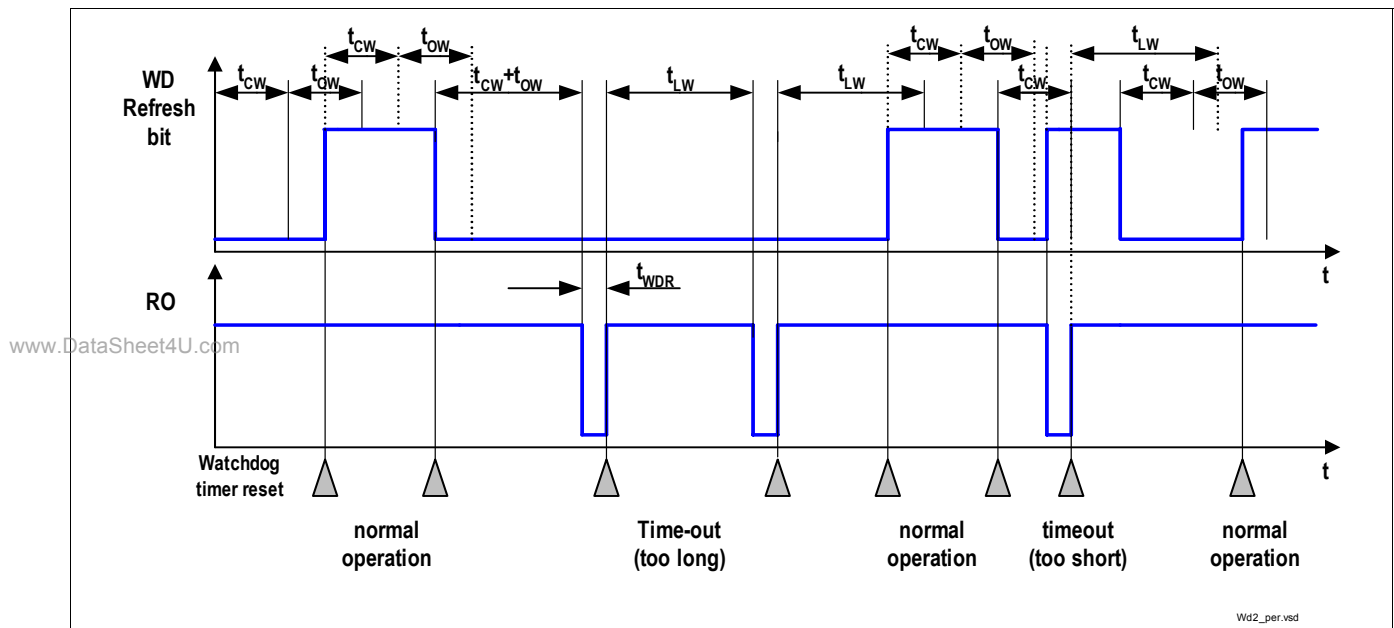
Figure 26 Window Watchdog Timing Diagram for config 1 and config 3
