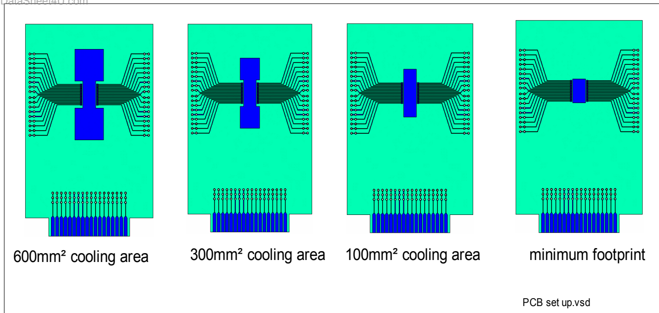
Figure 50 Board Set-up
