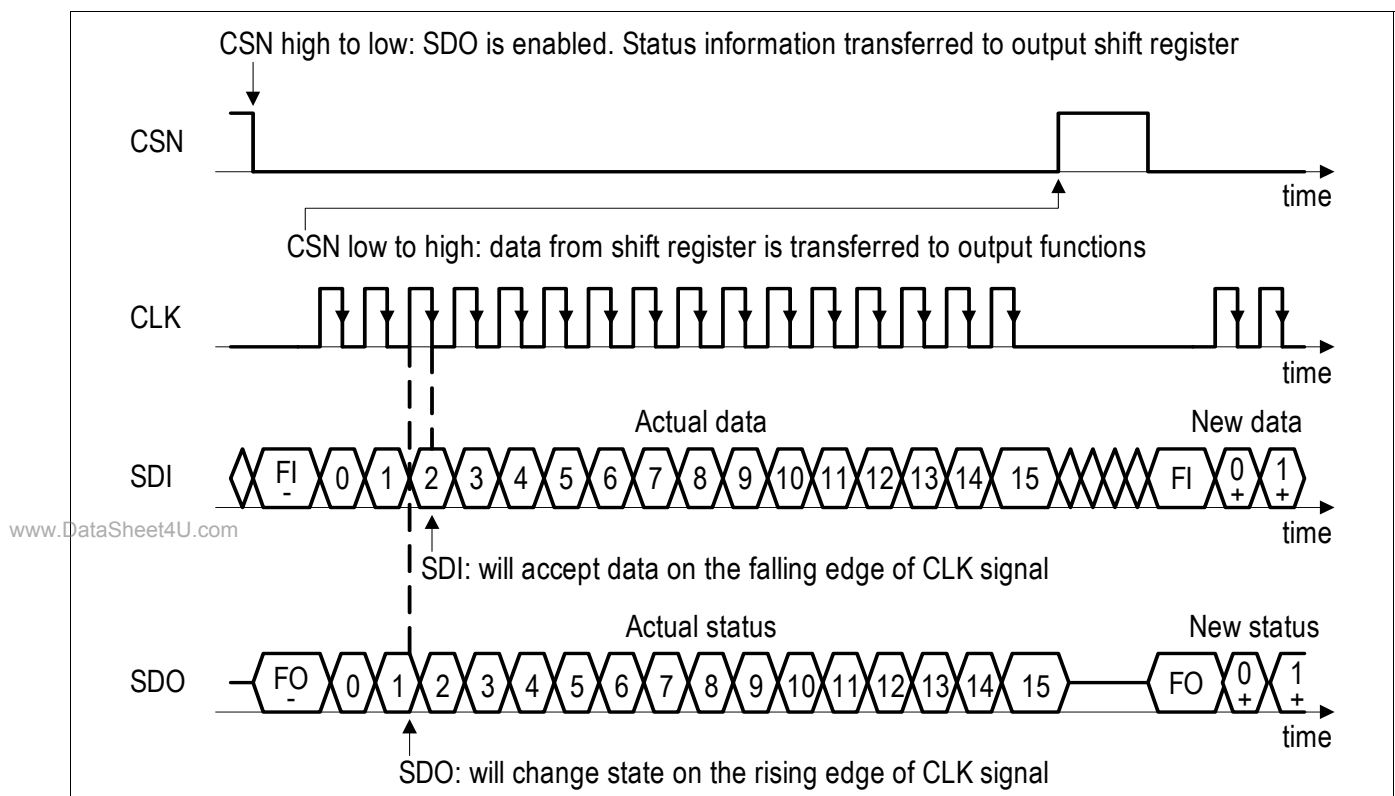
Figure 38 SPI Data Transfer Timing
