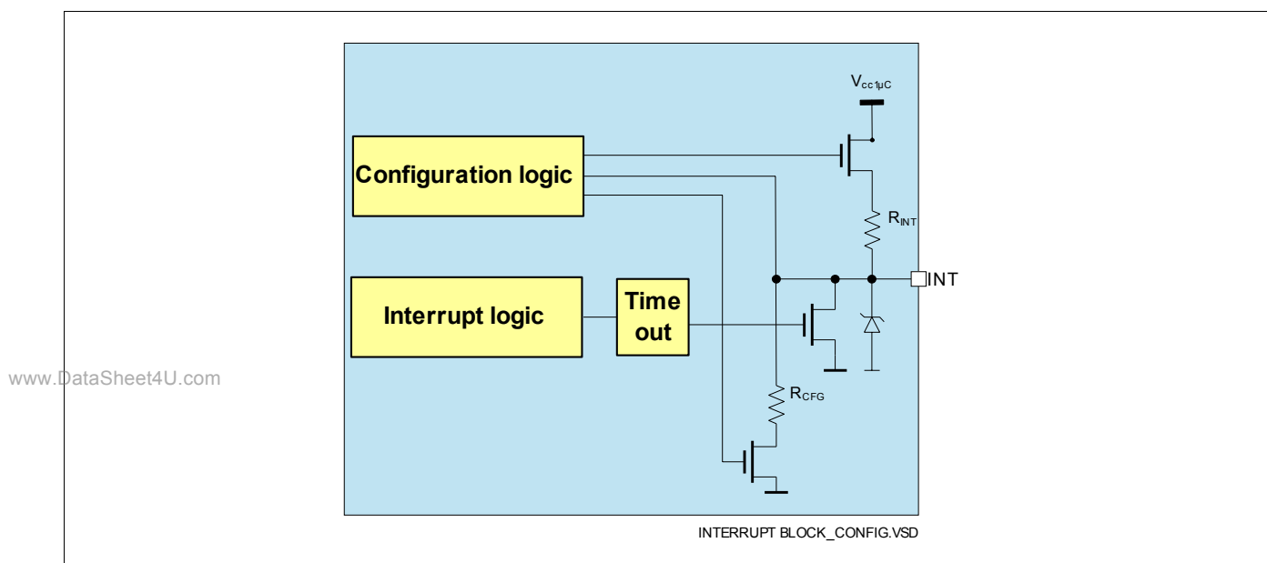
Figure 37 Config Logic Diagram
