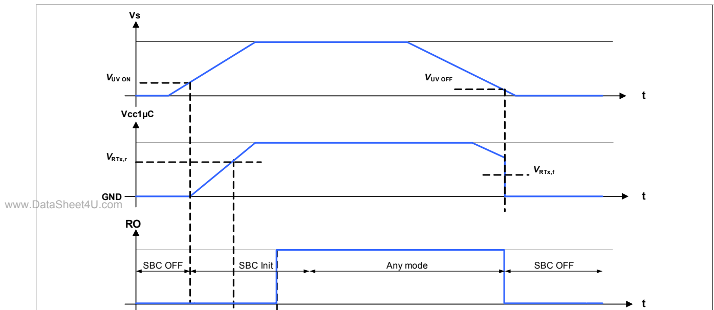
Figure 7 Ramp up / Down of Main Voltage Regulator
