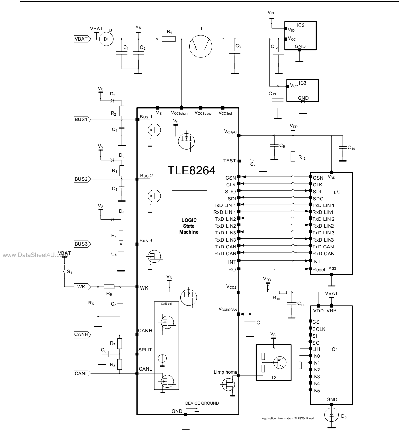
Figure 47 Application Example for a Body Controller Module
