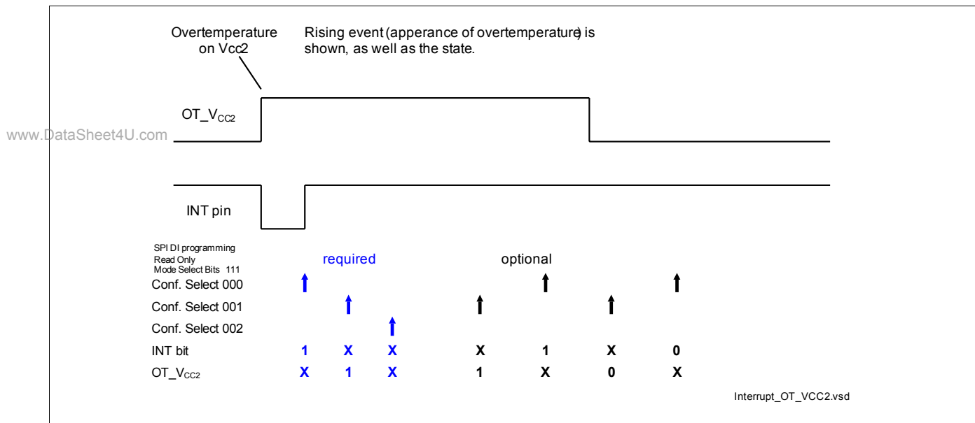
Figure 31 Interrupt V_{CC2} Over Temperature.
