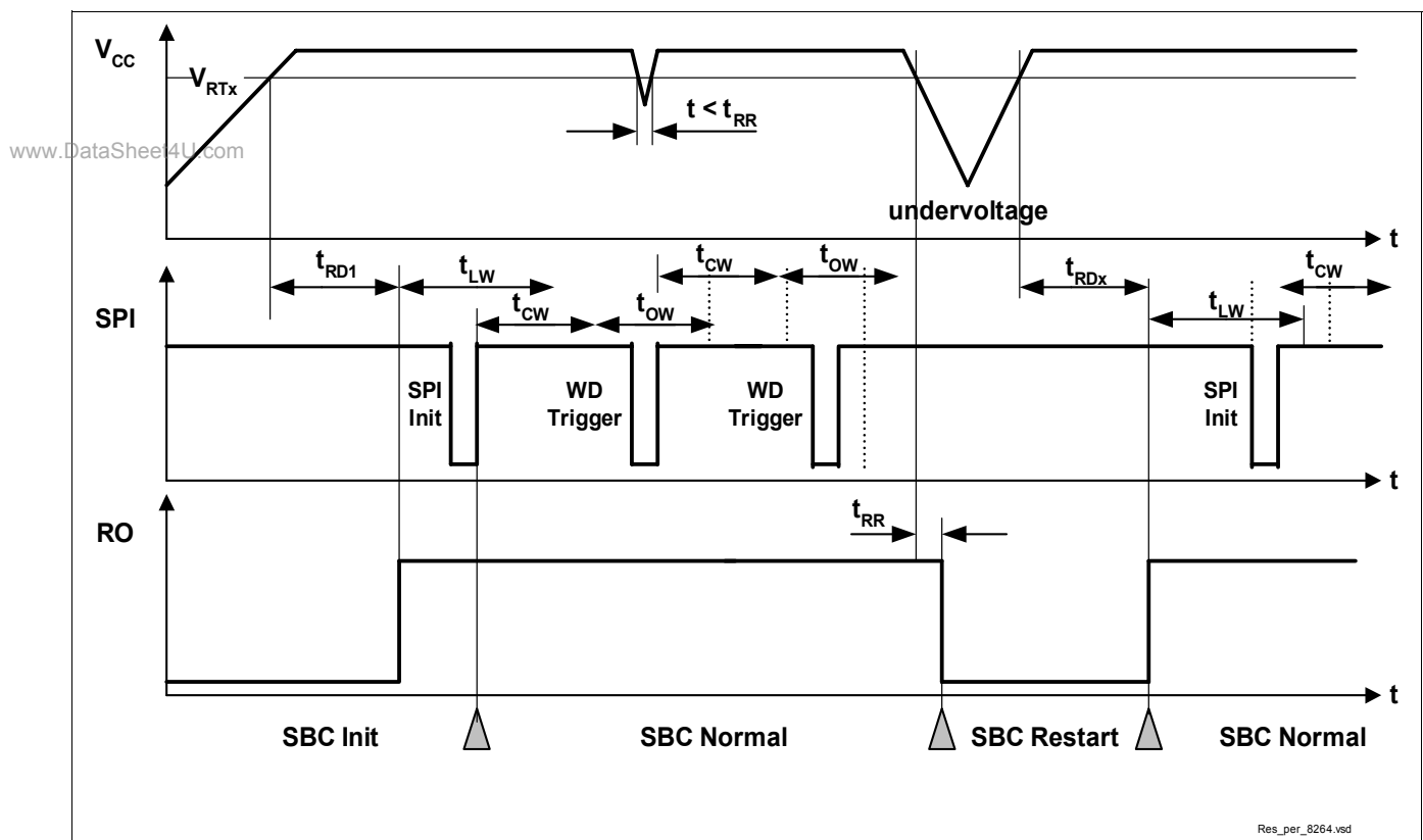
Figure 24 Reset Timing Diagram
