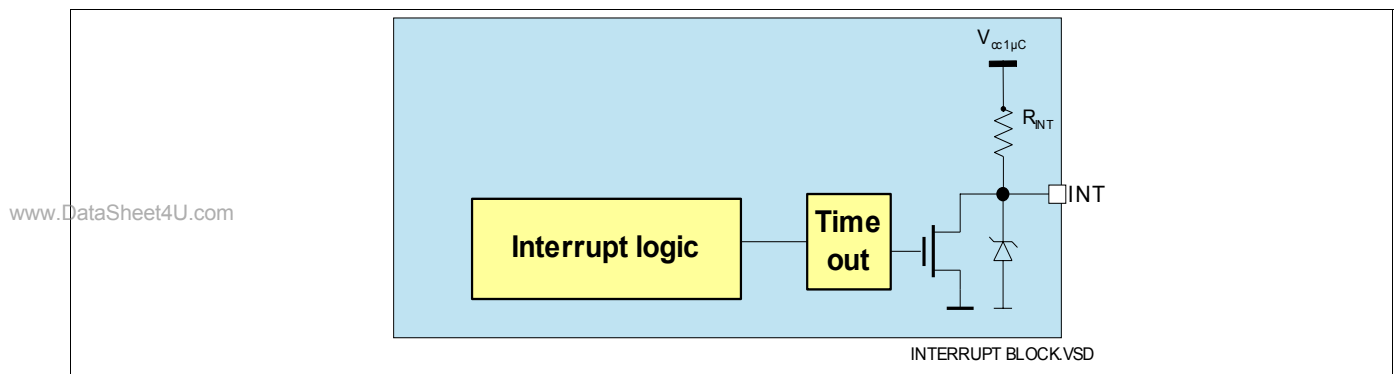
Figure 28 Interrupt Block Diagram
