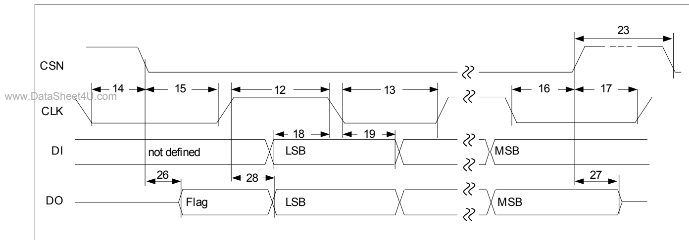
Figure 46 SPI Timing Diagram
