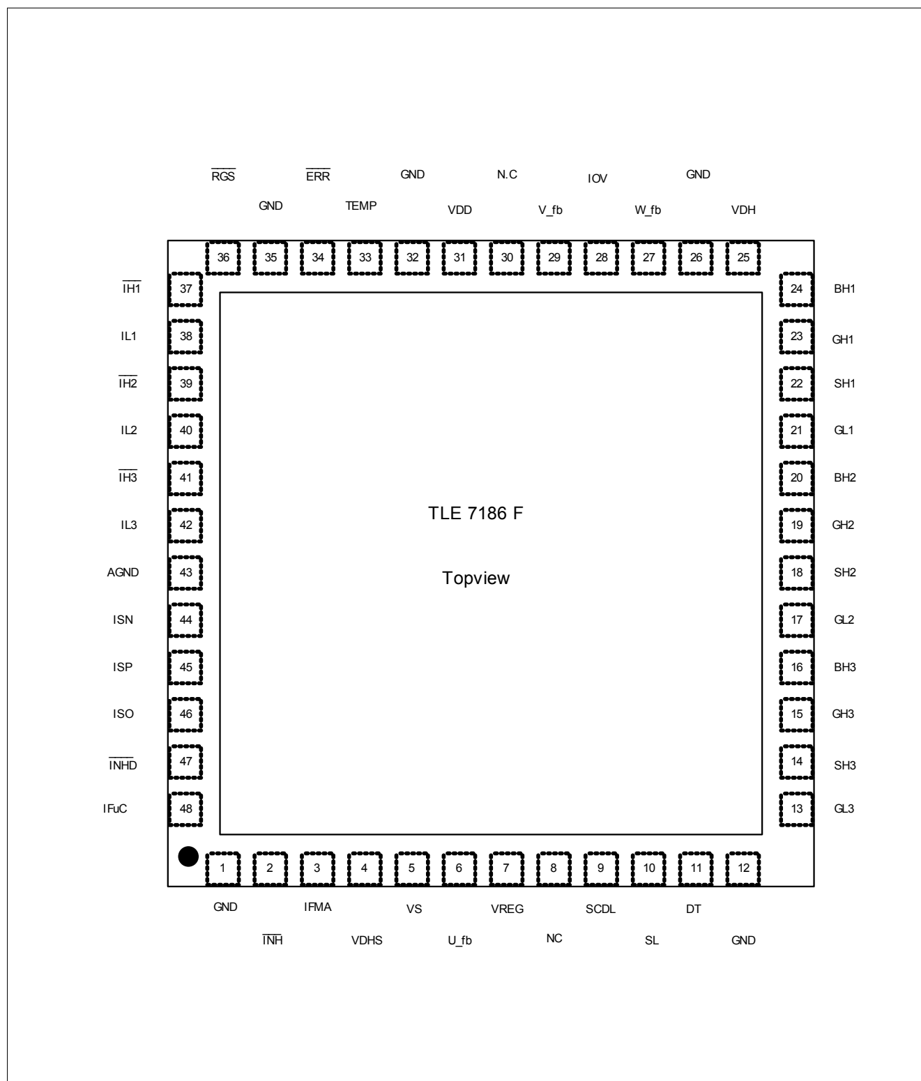
Figure 2 Pin Configuration
