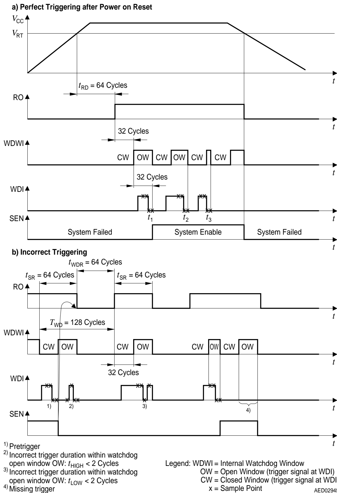
Figure 5 Window Watchdog Function
