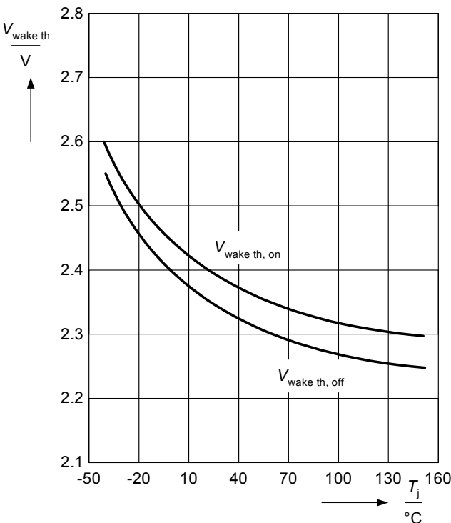
Device wake up thresholds vs. junction temperature
