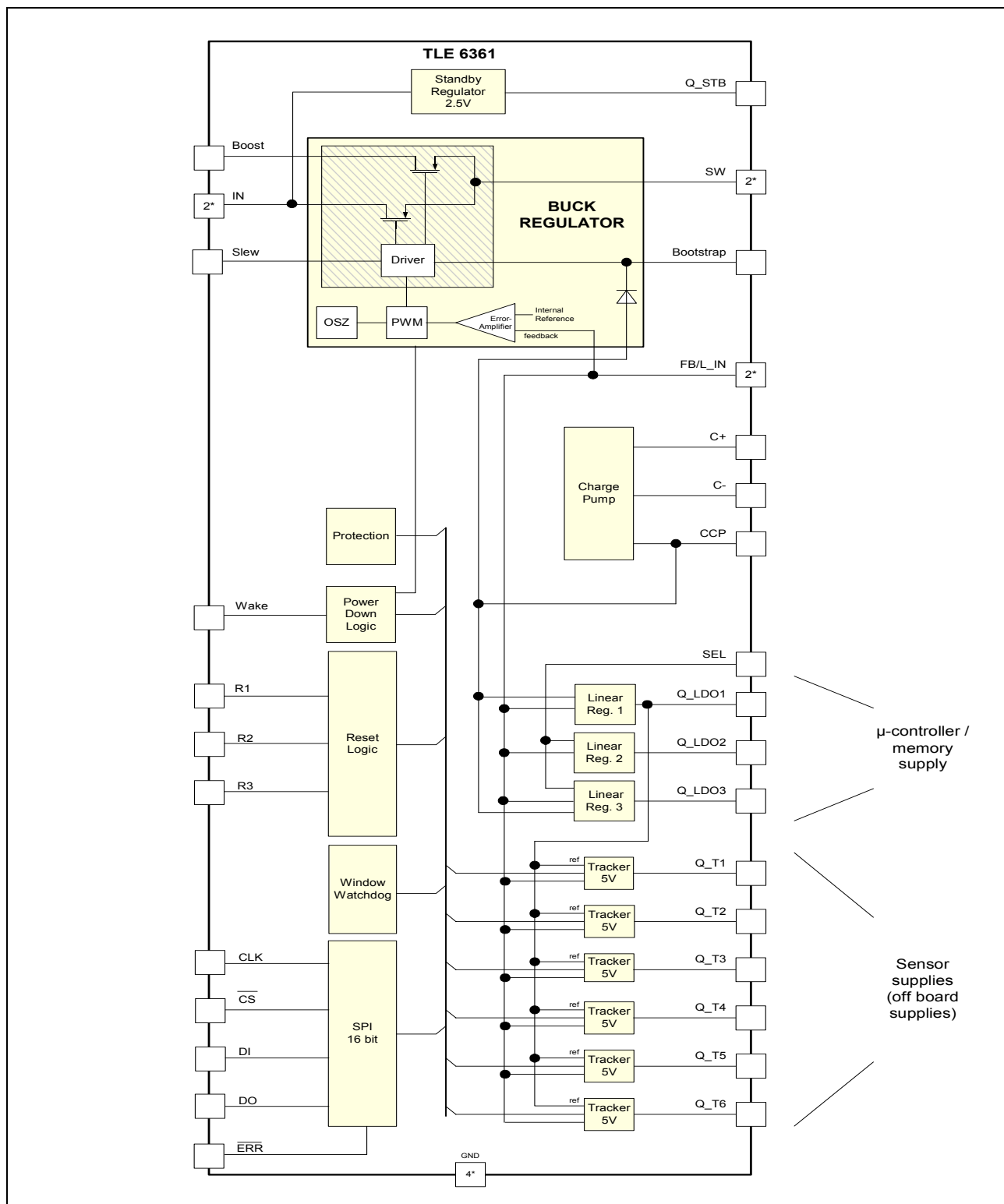
Figure 2 Block Diagram
