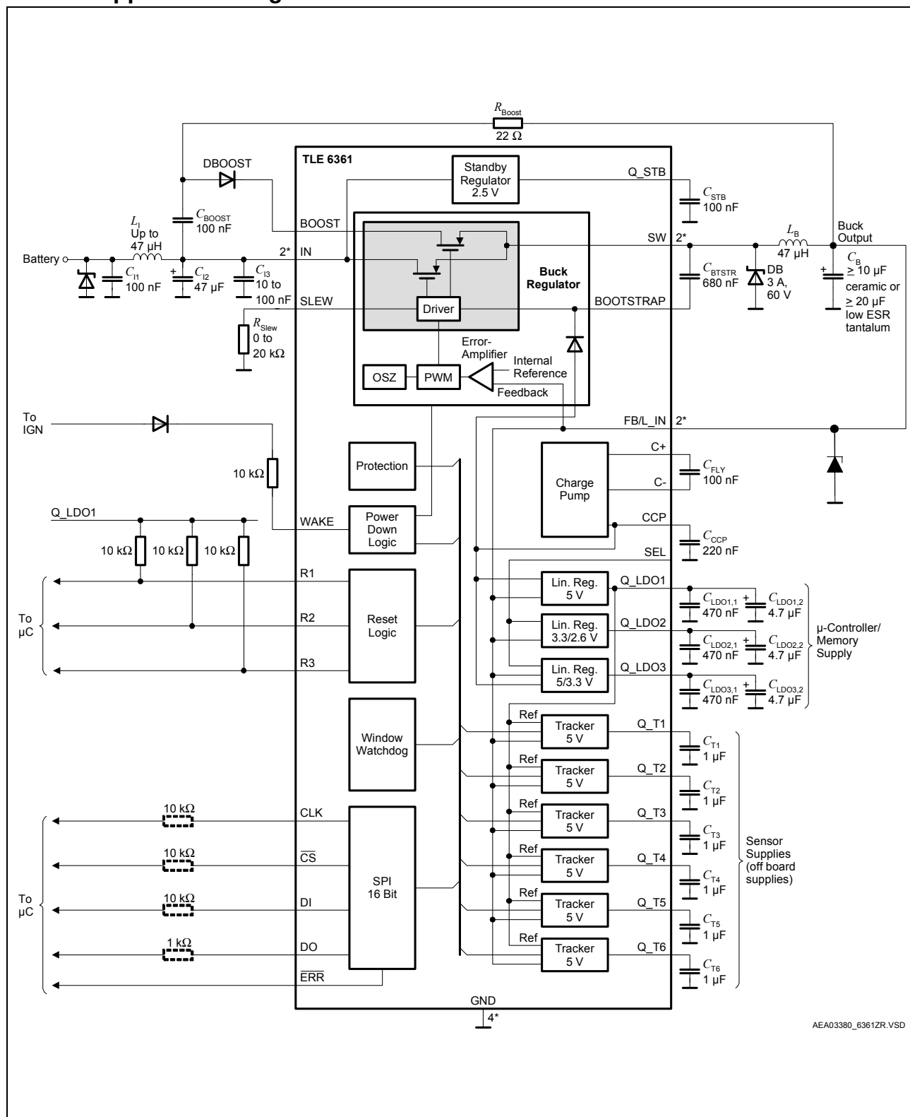
Figure 14 Application Diagram
