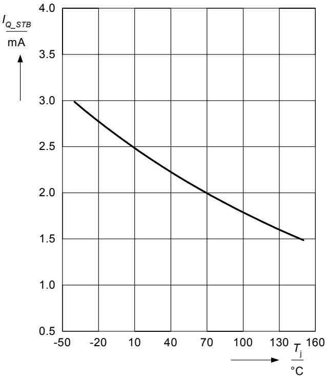
Q_STB current limit vs. junction temperature
