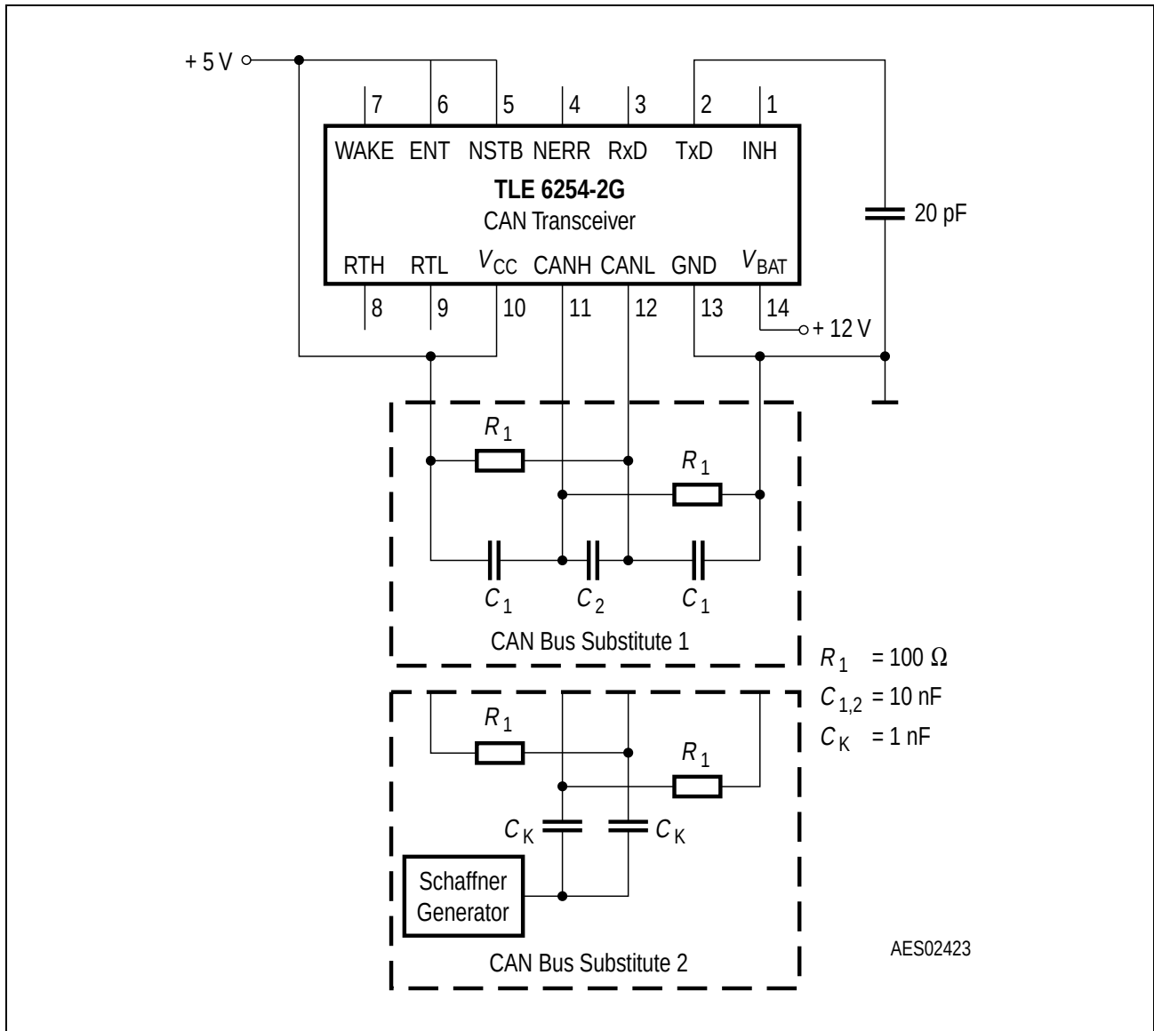
Figure 5 Test Circuits
