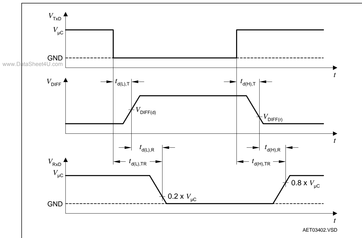
Figure 8 Timing Diagrams for Dynamic Characteristics
