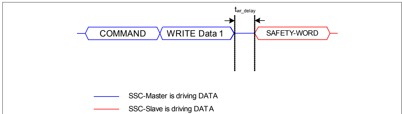
Figure 22 SSC data transfer (data-write example)
