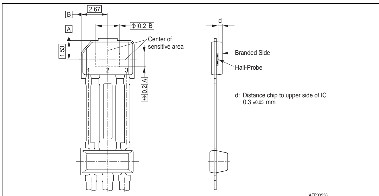
Figure 1 TLE4998P3C Pin Configuration and Hall Cell Location
