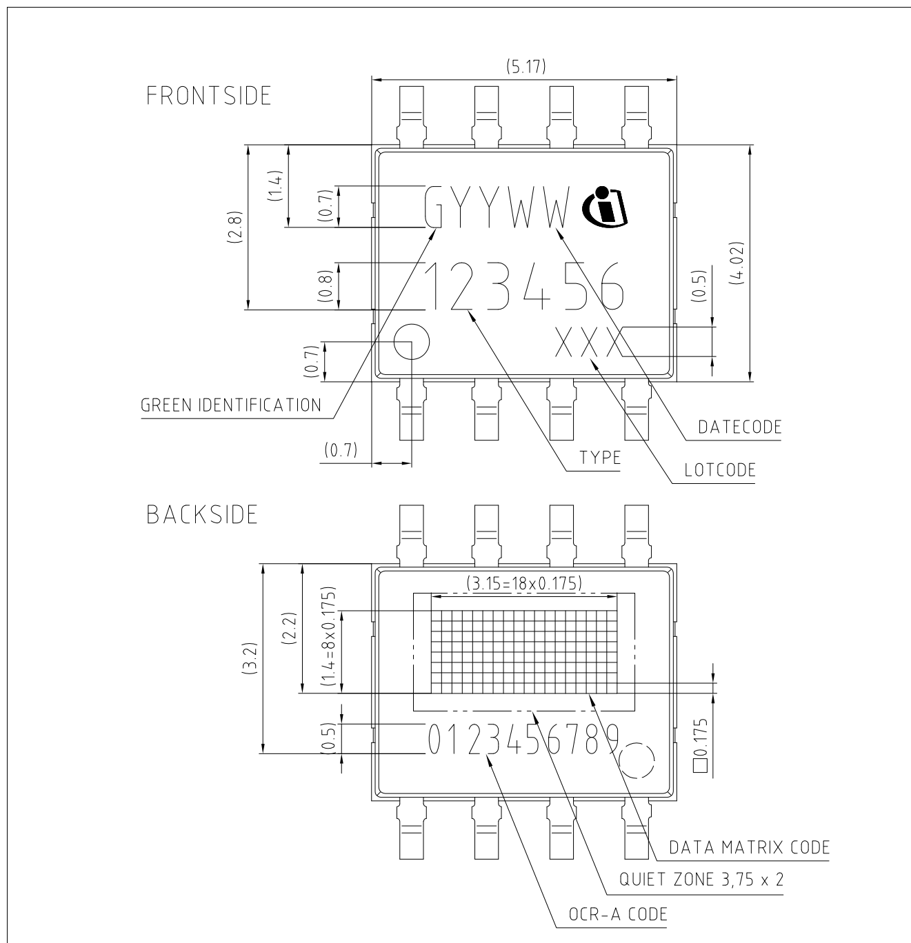
Figure 8-1 PG-TDSO-8-2 (PG-TDSO-Plastic G reen T hin D ual S mall O utline), Package Marking
