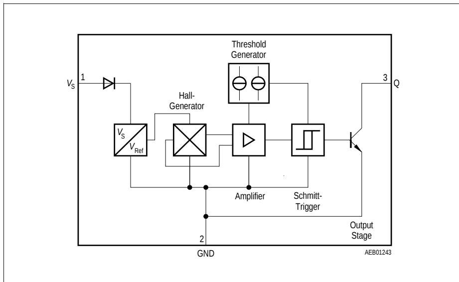
Figure 2 Block Diagram
