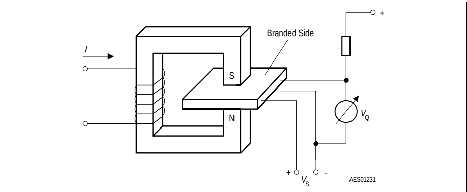
Figure 5 Sensor/Magnetic-Field Configuration
