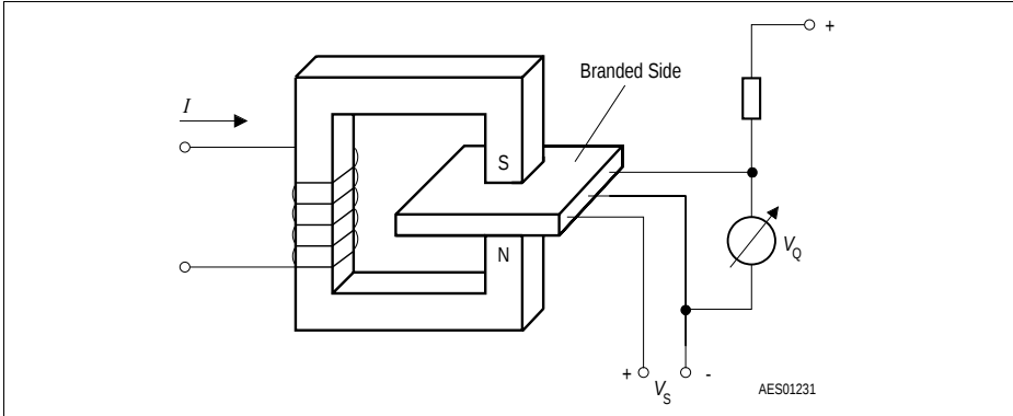
Figure 3 Sensor/Magnetic-Field Configuration
