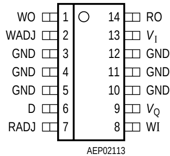
Figure 1 Pin Configuration (top view)
