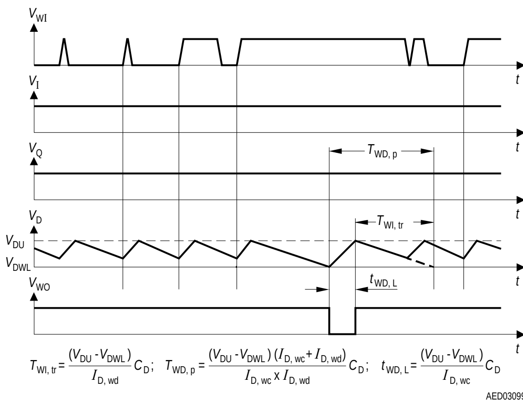
Figure 8 Timing of the Watchdog Function
