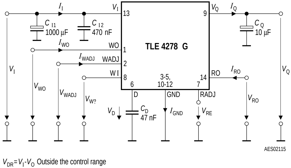
Figure 3 Test Circuit
