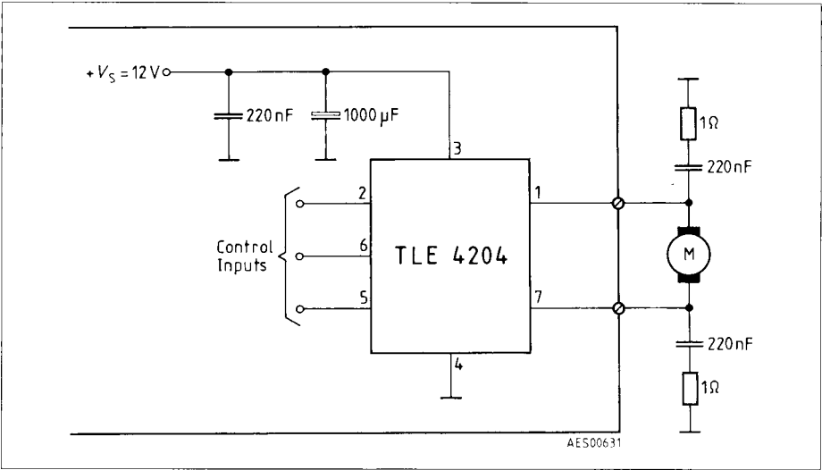
Figure 3 Application Circuit
