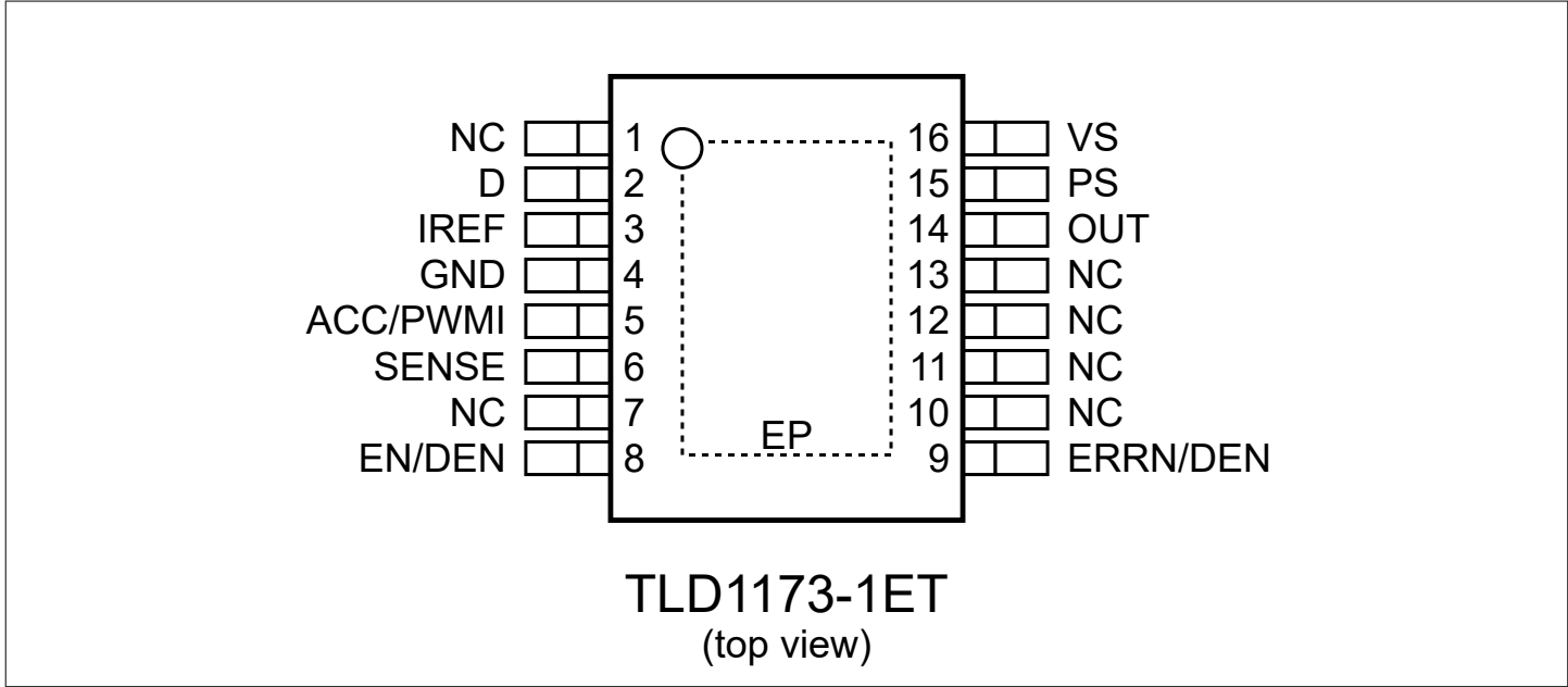
Figure 2 PG-TFDSO-16
