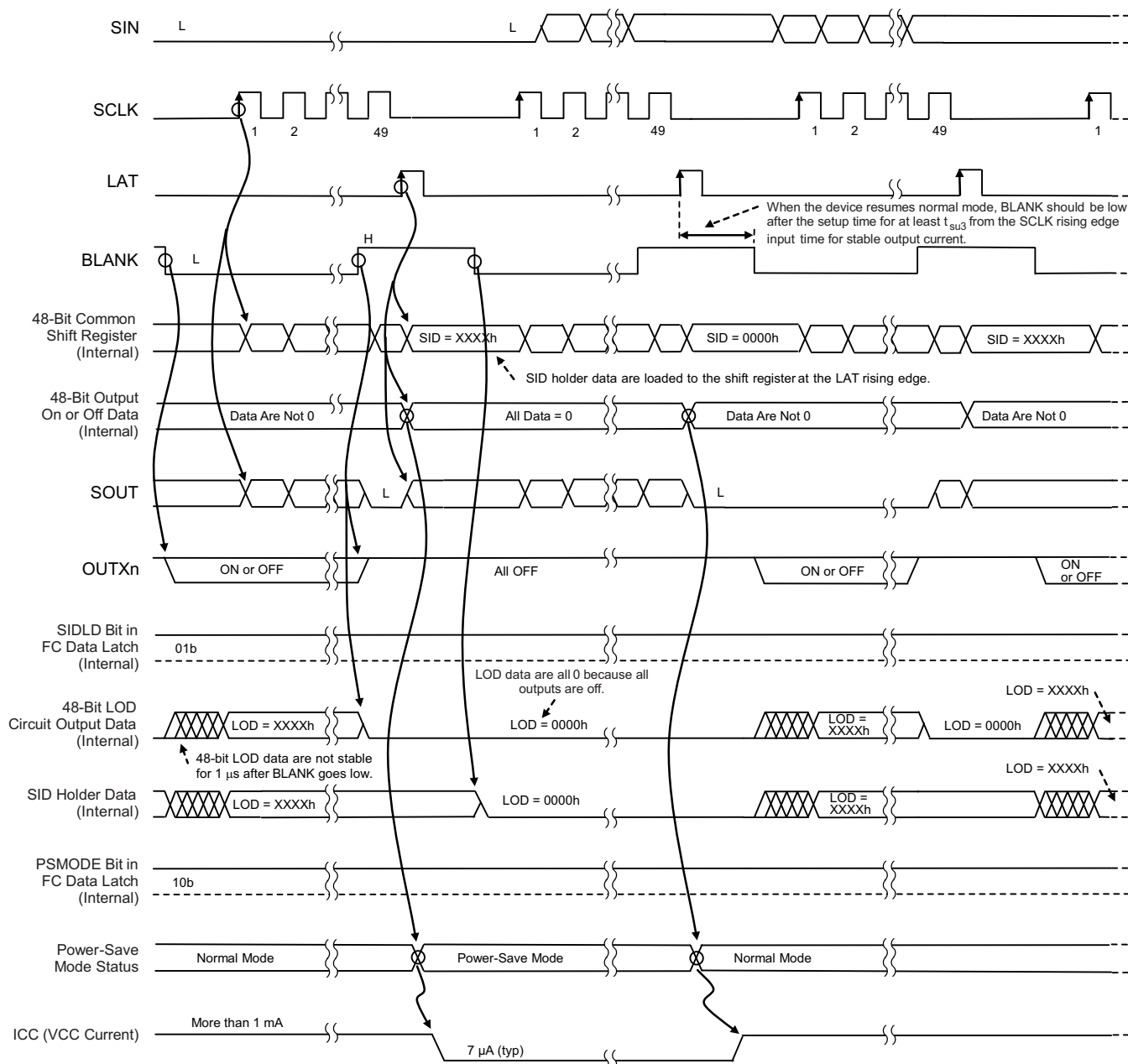
Figure 33. Power-Save Mode (FC Data PSMODE Bits = 10b)
