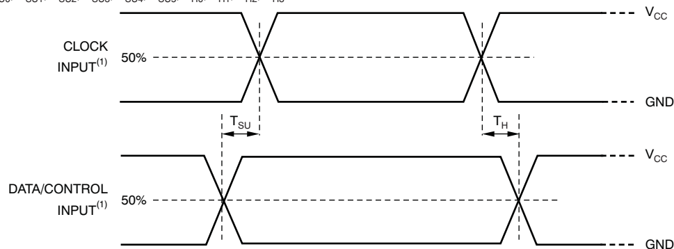
Figure 11. Input Timing
