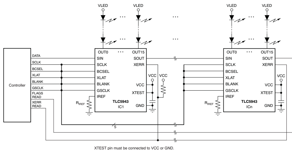
Typical Application Circuit (Multiple Daisy-Chained TLC5943s)
