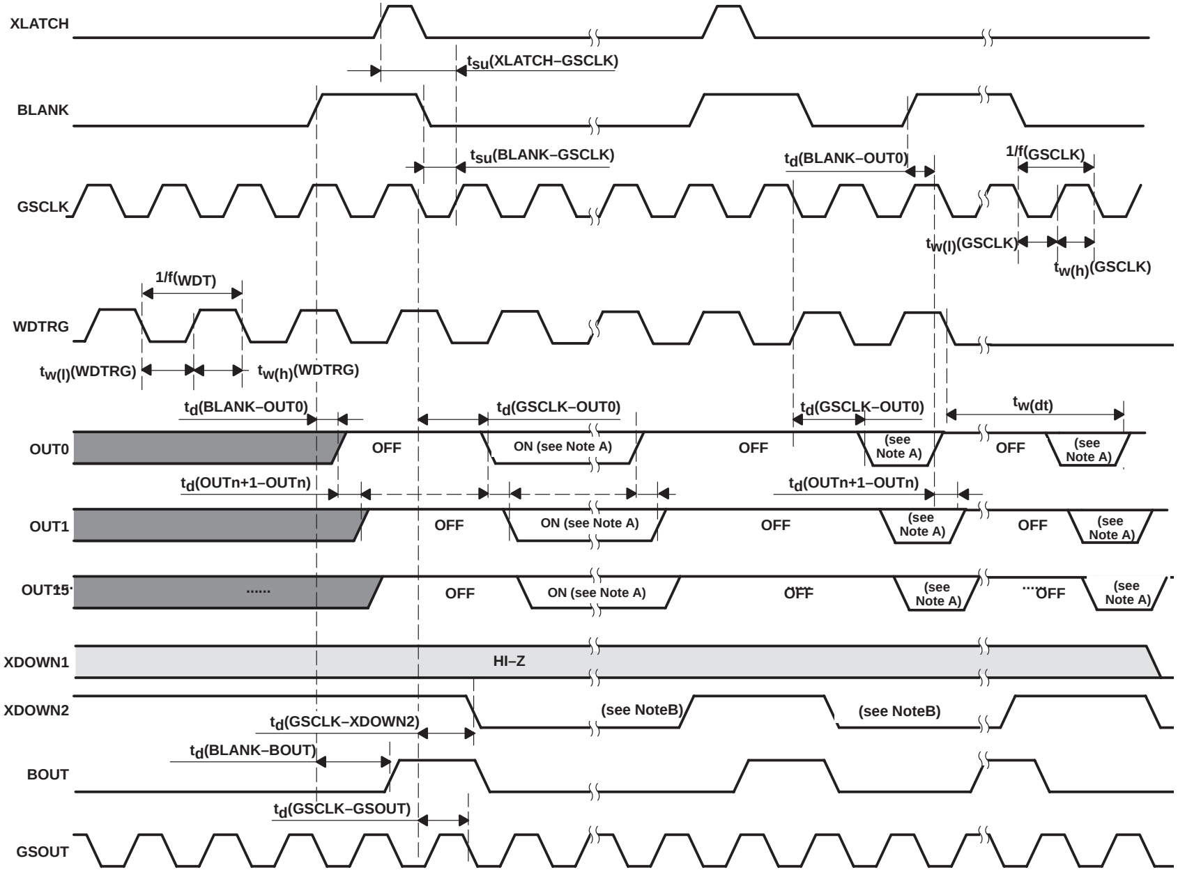
Figure 12. Timing Diagram (Constant Current Output)
