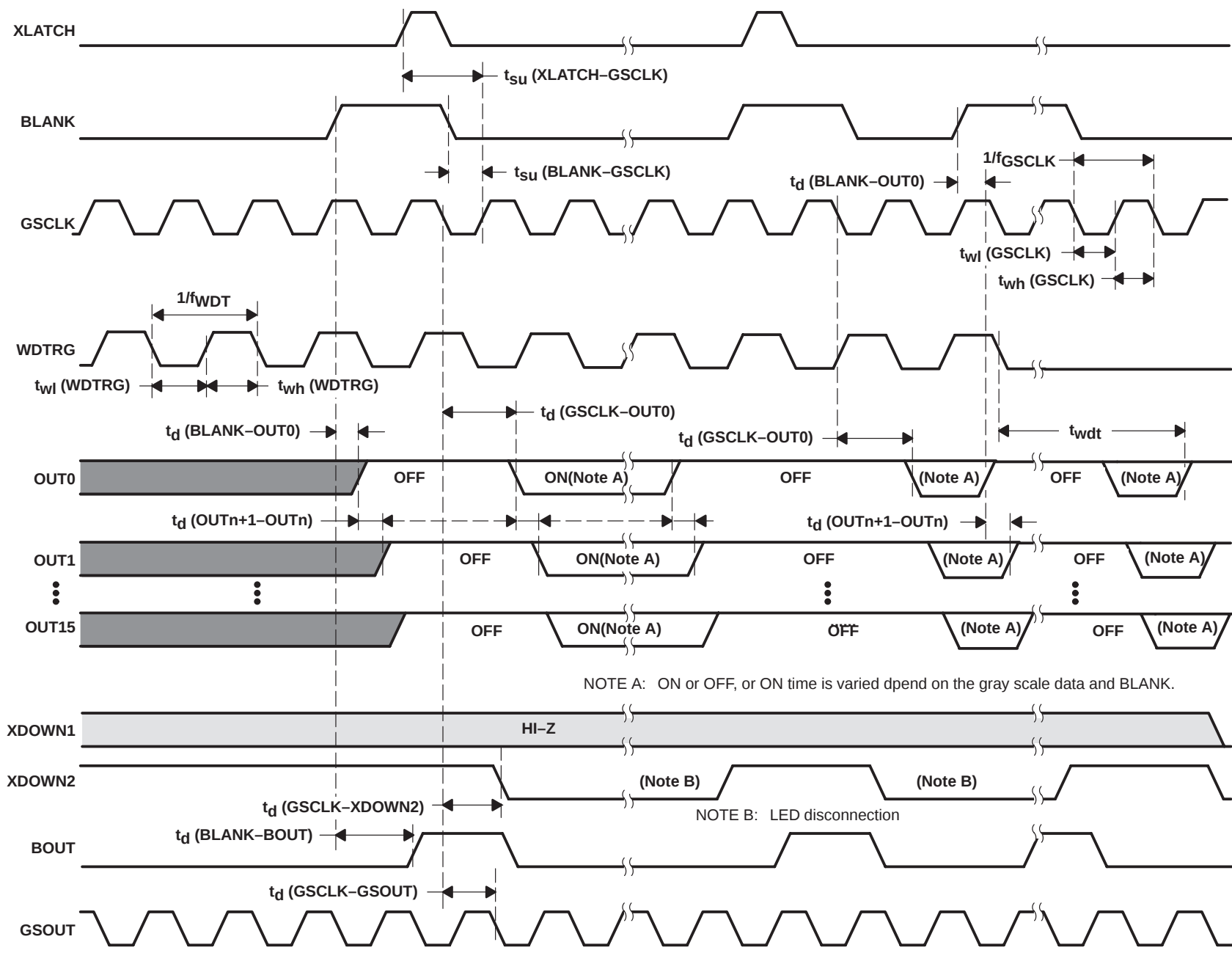
Figure 12. Timing Diagram (Constant Current Output)
