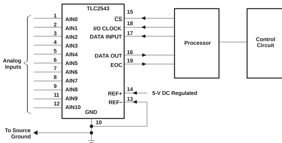
Figure 17. Serial Interface
