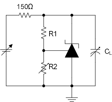
< Fig 4. Test Circuit >
