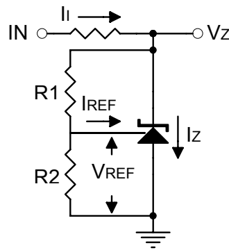
Fig 2. Test Circuit for V_Z>V_{REF} Note : V_Z=V_{REF}(1+R_1/R_2)+I_{REF}R_1
