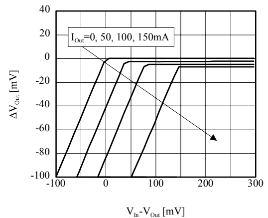
■ \Delta V_{\text{Out}} vs V_{\text{In}} (TK63128B)
