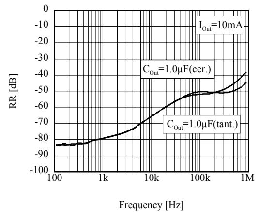
■ RR vs Frequency (TK63115B/H/S)
