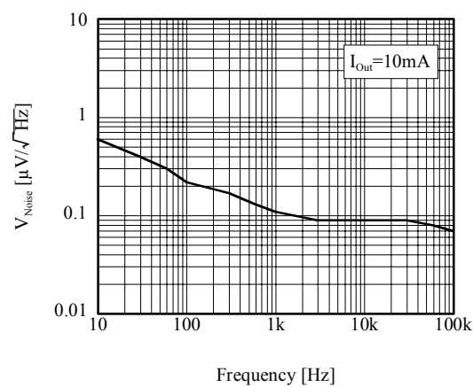
■ V_{\text{Noise}} vs Frequency (TK63115B/H/S)
