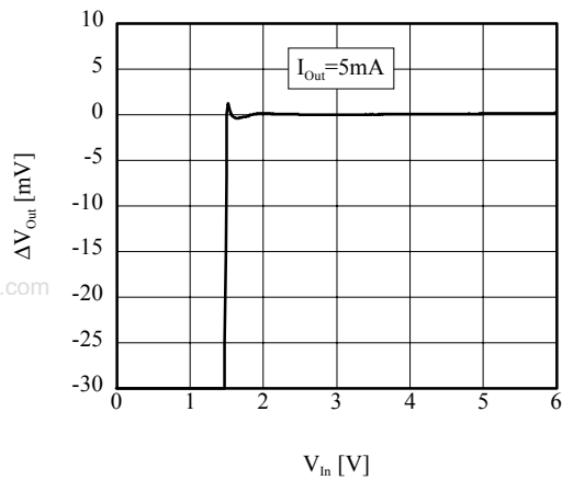
■ \Delta V_{\text{Out}} vs V_{\text{In}} (TK63115B/H/S)
