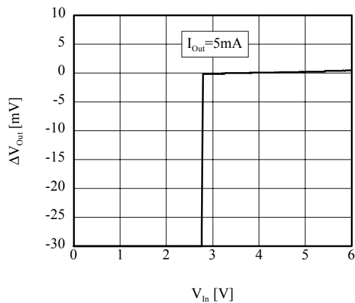
■ \Delta V_{\text{Out}} vs V_{\text{In}} (TK63128B/H/S)
