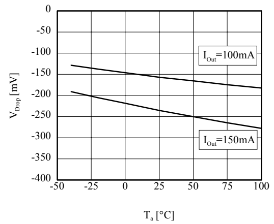
■ V_{\text{Drop}} vs T_a (TK63115B)
