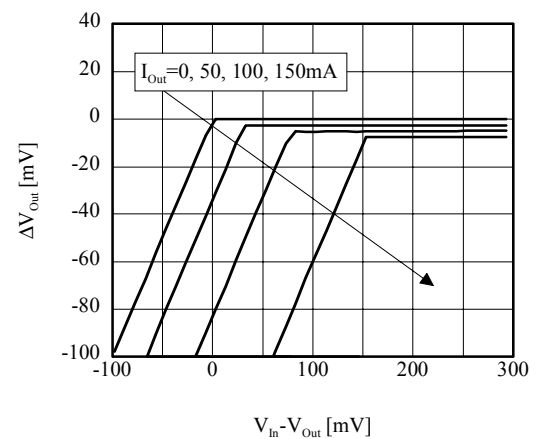
■ \Delta V_{\text{Out}} vs V_{\text{In}} (TK63142B)
