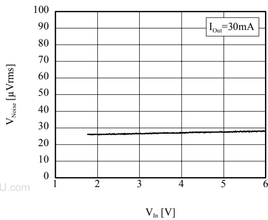
■ V_{\text{Noise}} vs V_{\text{In}} (TK63115B/H/S)
