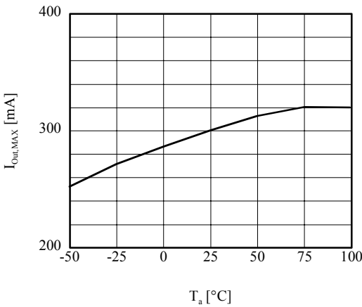
■ I_{Out,MAX} vs T_a (TK63128B/H/S)
