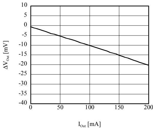
■ \Delta V_{Out} vs I_{Out} (TK63115H/S)
