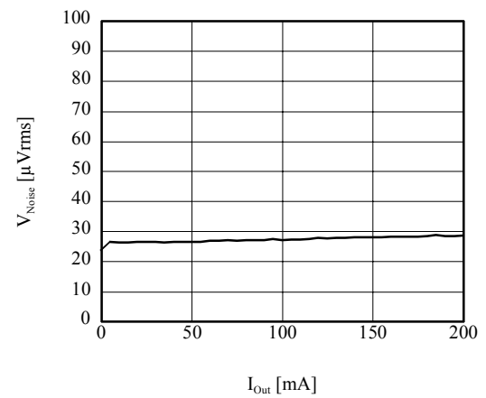
■ V_{\text{Noise}} vs I_{\text{Out}} (TK63115B/H/S)
