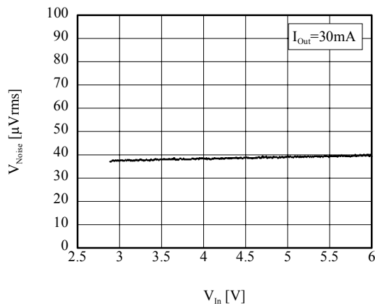
■ V_{\text{Noise}} vs V_{\text{In}} (TK63128B/H/S)
