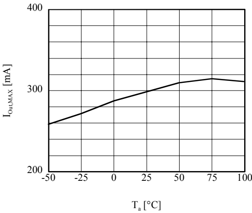
■ I_{Out,MAX} vs T_a (TK63142B/H/S)
