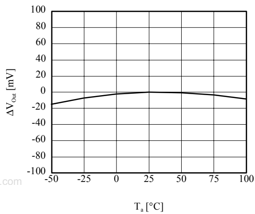
■ \Delta V_{\text{Out}} vs T_a (TK63115B/H/S)
