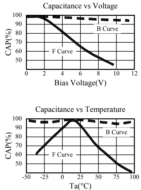
Fig12-4: ex. Ceramic Capacitance vs Voltage, Temperature
