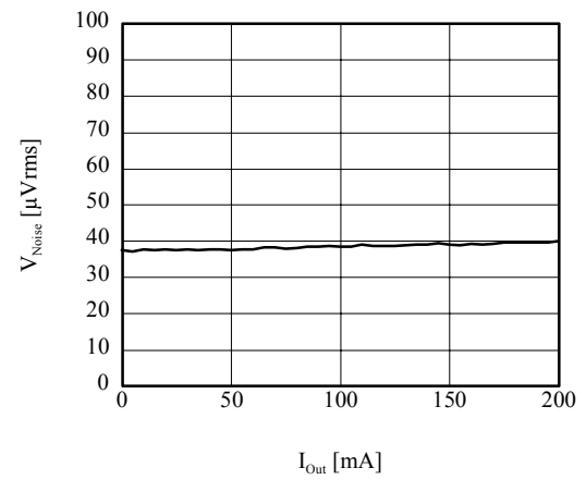
■ V_{\text{Noise}} vs I_{\text{Out}} (TK63128B/H/S)
