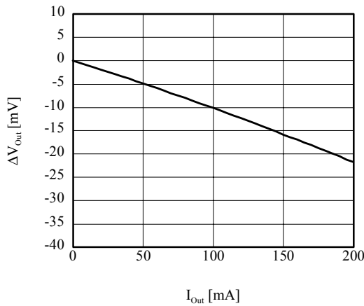
■ \Delta V_{Out} vs I_{Out} (TK63128H/S)
