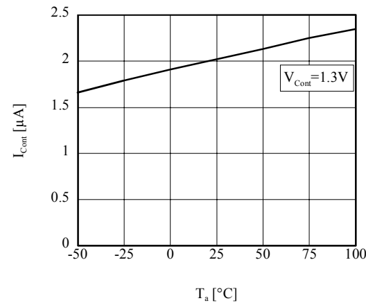
■ I_{Cont} vs T_a (TK631xxB/H/S)
