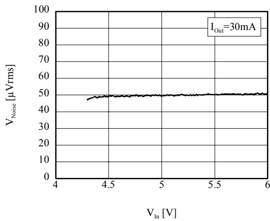
■ V_{\text{Noise}} vs V_{\text{In}} (TK63142B/H/S)
