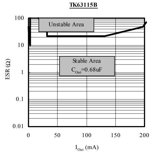
Fig12-2: Output Current vs Stable Operation Area (TK631xxB)
