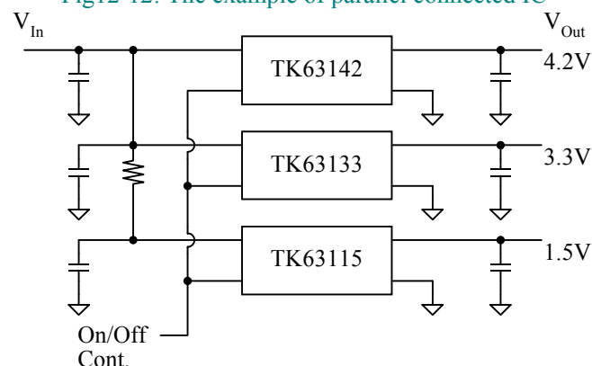
Fig12-12: The example of parallel connected IC
