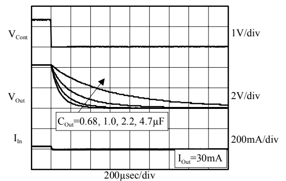
■ On/Off Transient ( V_{Cont}=1.3 \rightarrow 0V ) (TK63142B/H/S)
