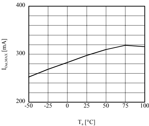
■ I_{Out,MAX} vs T_a (TK63115B/H/S)
