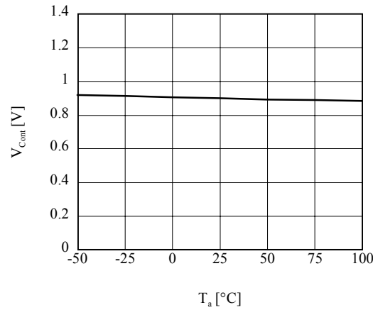
■ V_{Cont} vs T_a (TK63142B/H/S)
