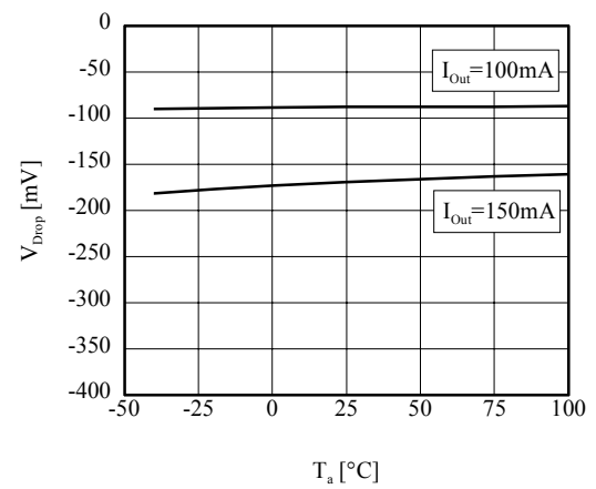
■ V_{\text{Drop}} vs T_a (TK63142B)
