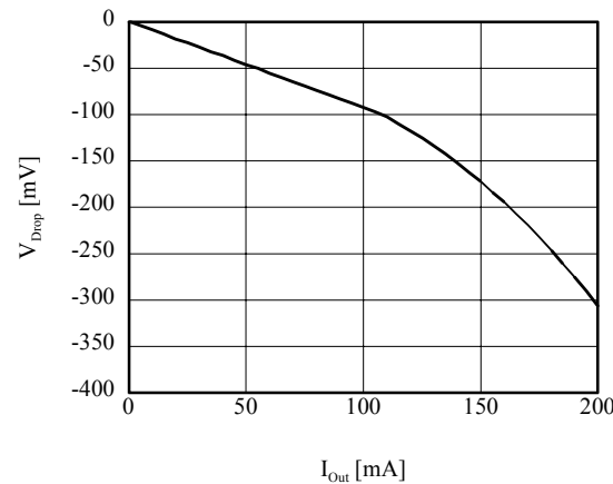
■ V_{Drop} vs I_{Out} (TK63128H/S)
