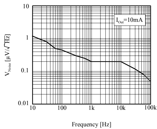
■ V_{\text{Noise}} vs Frequency (TK63128B/H/S)
