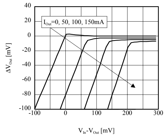
■ \Delta V_{\text{Out}} vs V_{\text{In}} (TK63115B)
