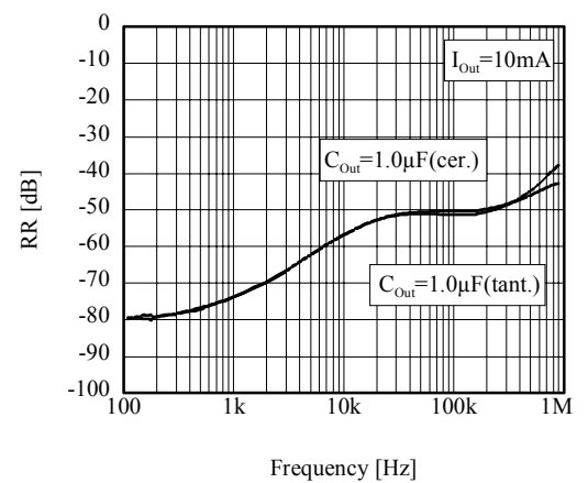
■ RR vs Frequency (TK63142B/H/S)
