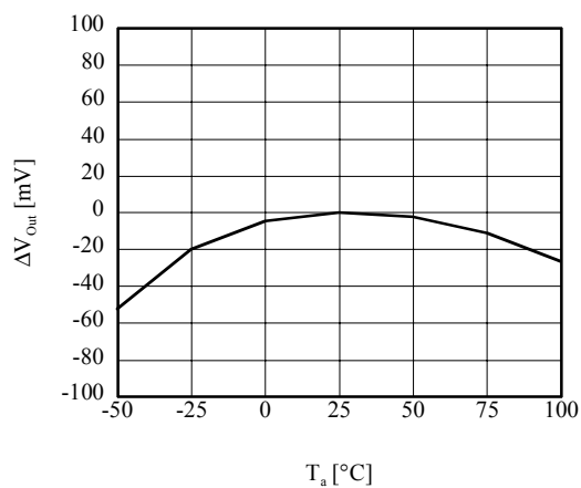
■ \Delta V_{\text{Out}} vs T_a (TK63142B/H/S)
