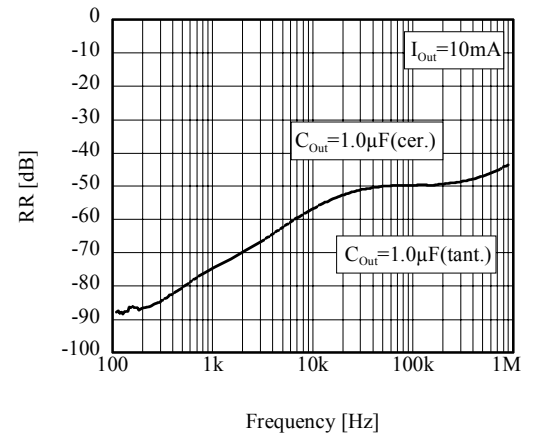
■ RR vs Frequency (TK63128B/H/S)
