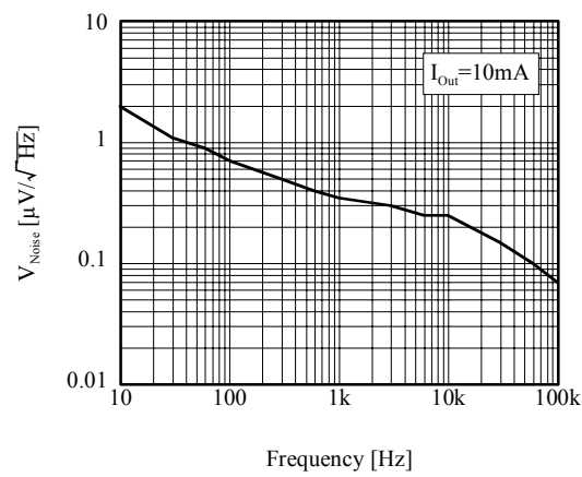
■ V_{\text{Noise}} vs Frequency (TK63142B/H/S)
