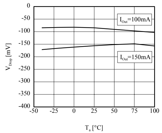
■ V_{\text{Drop}} vs T_a (TK63128B)
