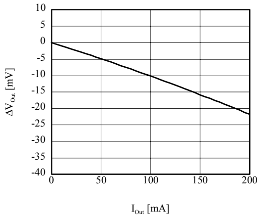
■ \Delta V_{Out} vs I_{Out} (TK63142H/S)
