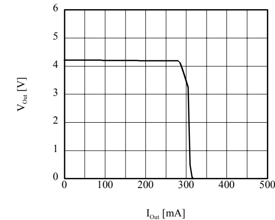
■ V_{Out} vs I_{Out} (TK63142B/H/S)
