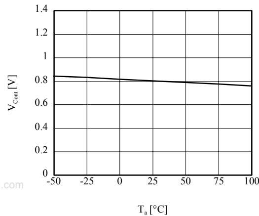
■ V_{Cont} vs T_a (TK63115B/H/S)
