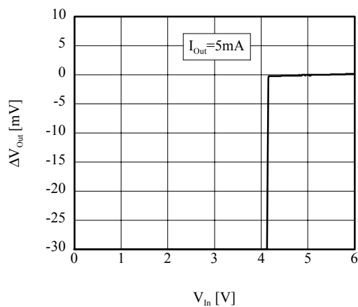
■ \Delta V_{\text{Out}} vs V_{\text{In}} (TK63142B/H/S)
