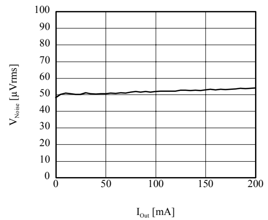
■ V_{\text{Noise}} vs I_{\text{Out}} (TK63142B/H/S)
