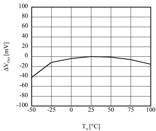
■ \Delta V_{\text{Out}} vs T_a (TK63128B/H/S)
