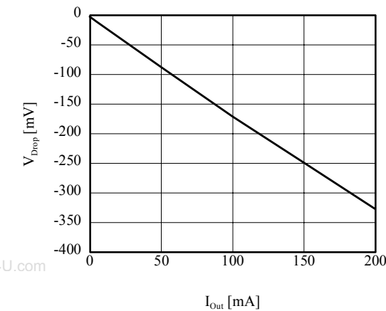
■ V_{Drop} vs I_{Out} (TK63115H/S)
