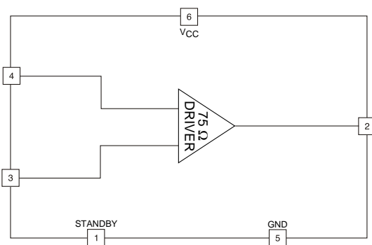
BLOCK DIAGRAM
