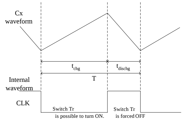
Figure 1: OSC Waveforms
