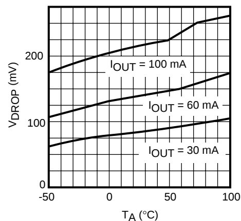
DROPOUT VOLTAGE
