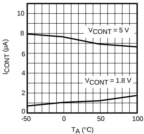
CONTROL CURRENT
