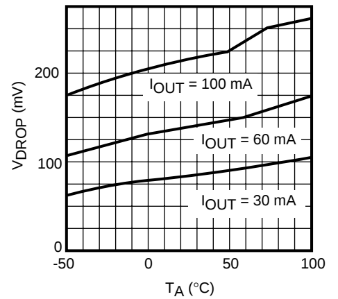
DROPOUT VOLTAGE
