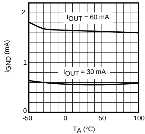
GROUND CURRENT
