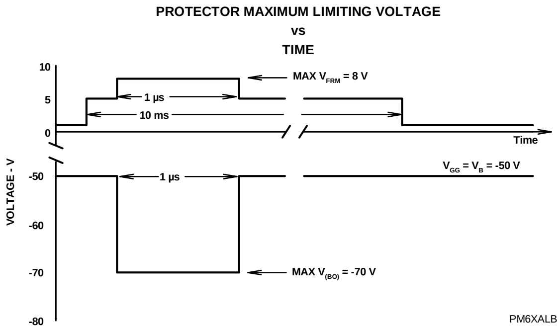
Figure 2 TRANSIENT LIMITS FOR TISPPBLx LIMITING VOLTAGE
