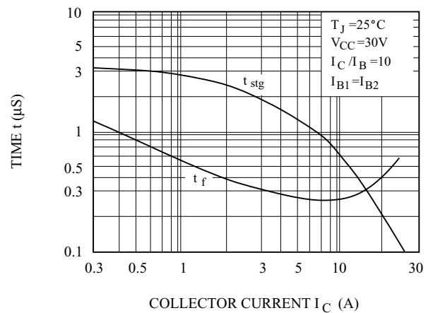
SWITCHING CHARACTERISTICS
