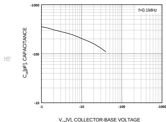
Figure 4. Collector Output Capacitance
